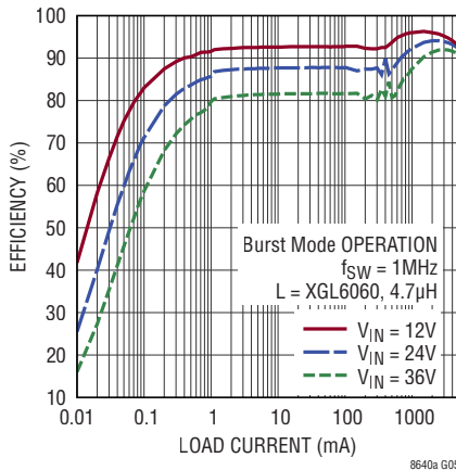
Low Load Efficiency at 5V OUT
