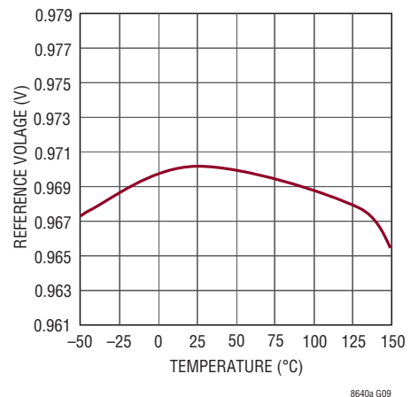
LT8640A Feedback Reference Voltage
