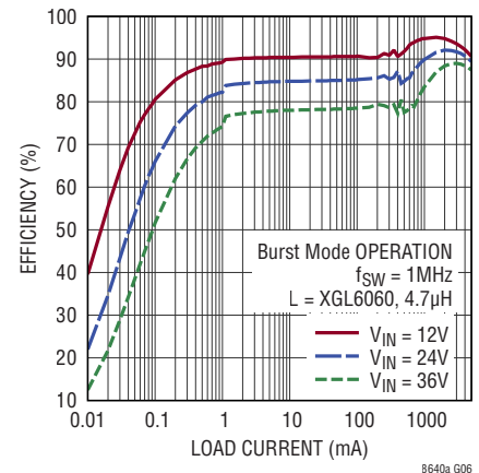
Low Load Efficiency at 3.3V OUT
