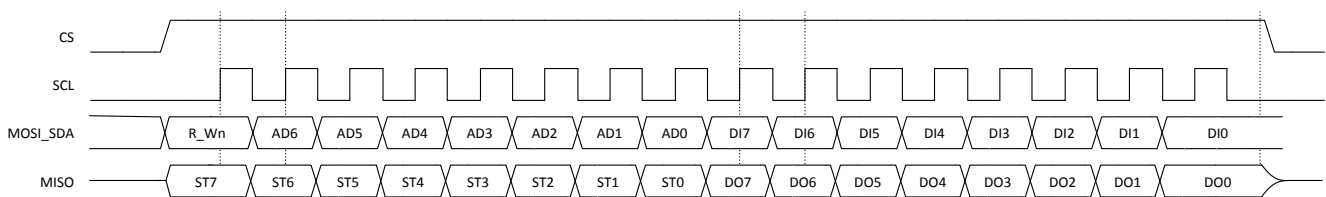
Figure 7-4 SPI transaction scheme CPOL=0, CPHA=0
