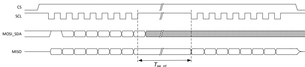
Figure 7-6 SPI transaction for reading the E 2 PROM (CPOL=1)
