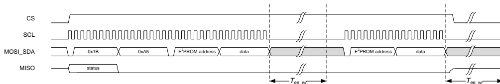
Figure 7-9 SPI multi-byte transaction for writing the E 2 PROM
