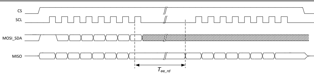
Figure 7-7 SPI transaction for reading the E 2 PROM (CPOL=0)
