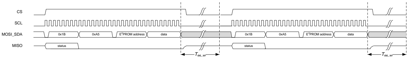
Figure 7-8 Two consecutive single E 2 PROM write SPI transactions
