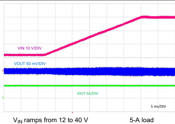
Figure 9-33. Line Transient Response to V_{IN} = 40\text{ V}
