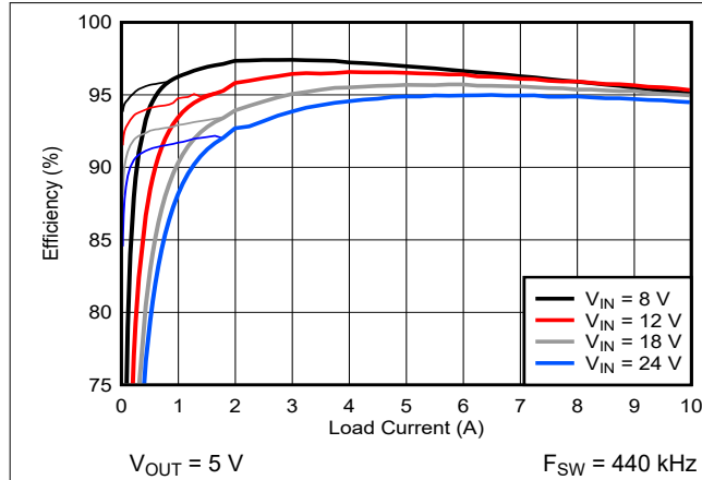
Figure 7-1. Efficiency vs Load
