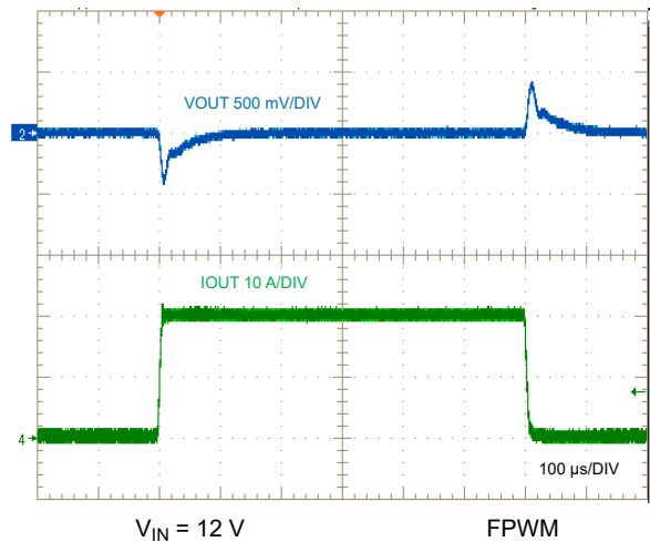
Figure 9-45. Load Transient, 0 A to 20 A
