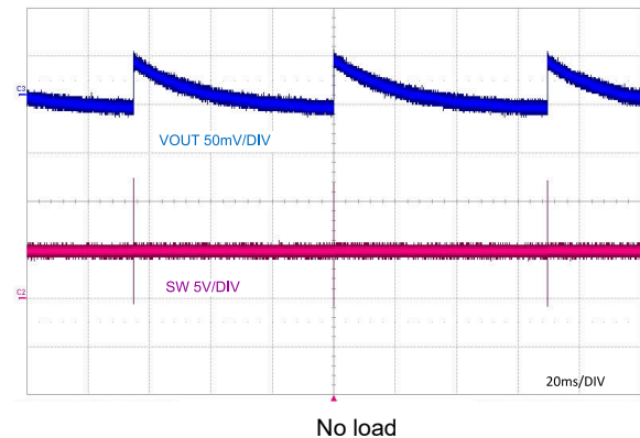
Figure 9-8. PFM Switching
