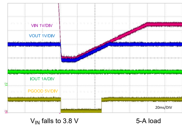
Figure 9-10. Cold-Crank Response to V_{IN} = 3.8\text{ V}
