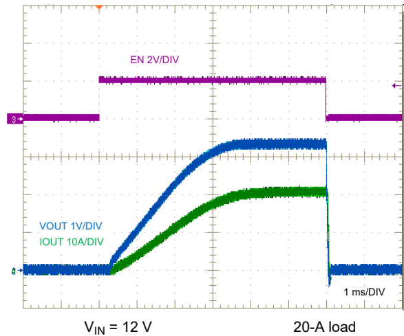
Figure 9-43. ENABLE ON and OFF Characteristic
