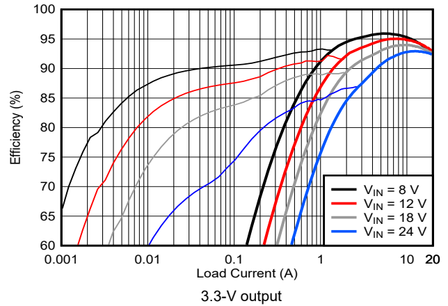
Figure 9-41. Efficiency vs I_{OUT} , Log Scale
