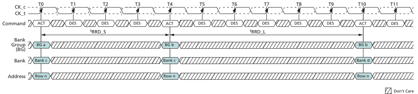
Figure 121: t_{RRD} Timing
