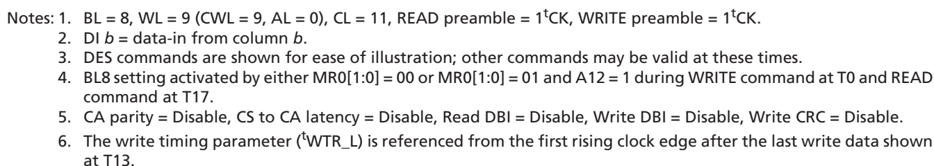
Figure 185: WRITE (BC4) OTF to READ (BC4) OTF with 1 st CK Preamble in Different Bank Group
