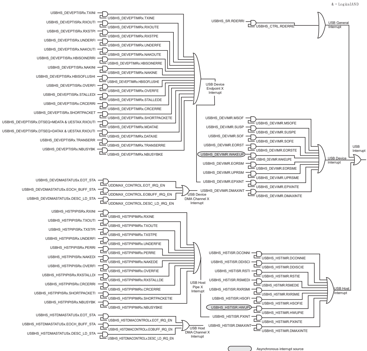
Figure 38-3. Interrupt System
