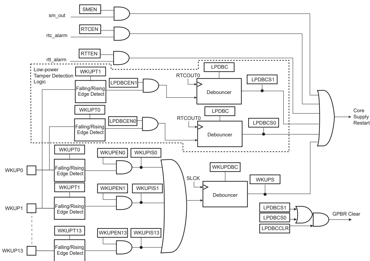
Figure 23-7. Wakeup Sources
