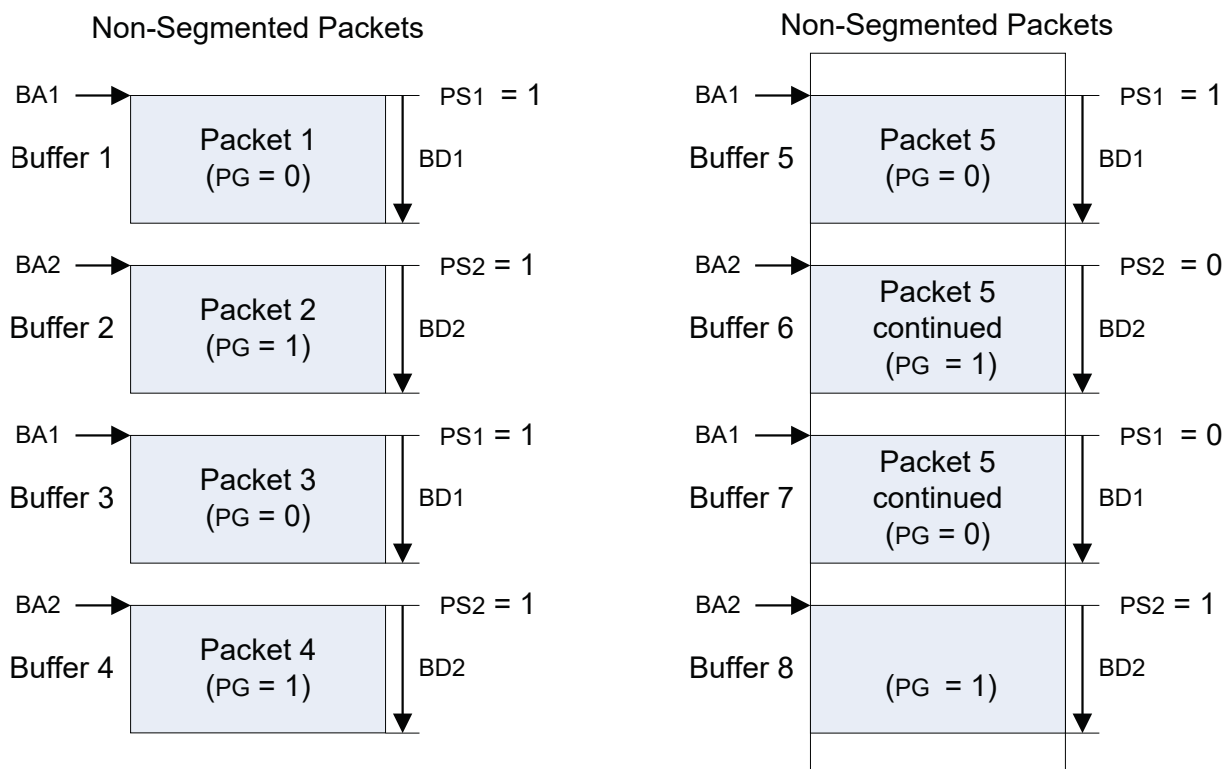
Figure 47-22. Single-packet Asynchronous or Control System Memory Structure
