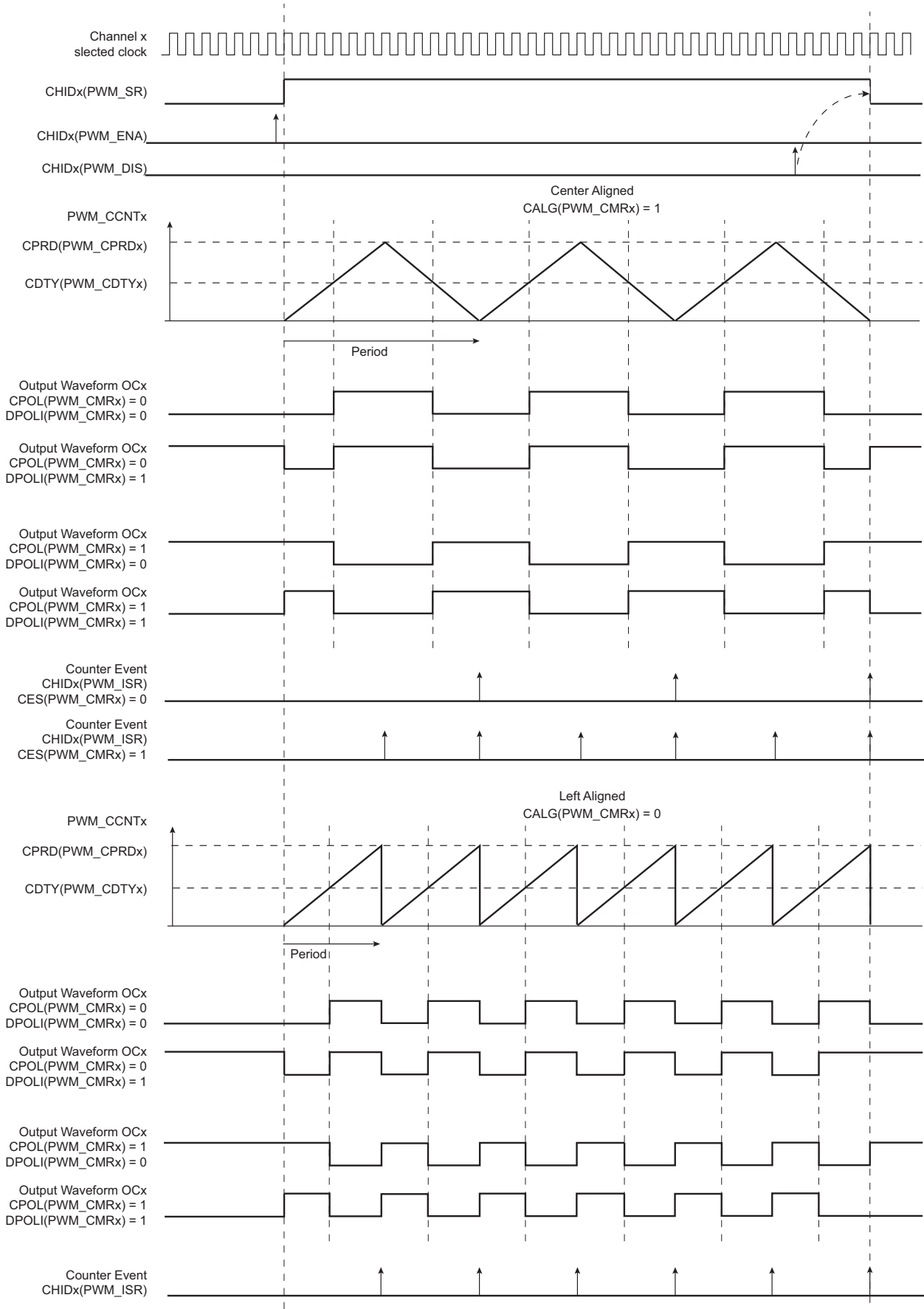
Figure 50-5. Waveform Properties
