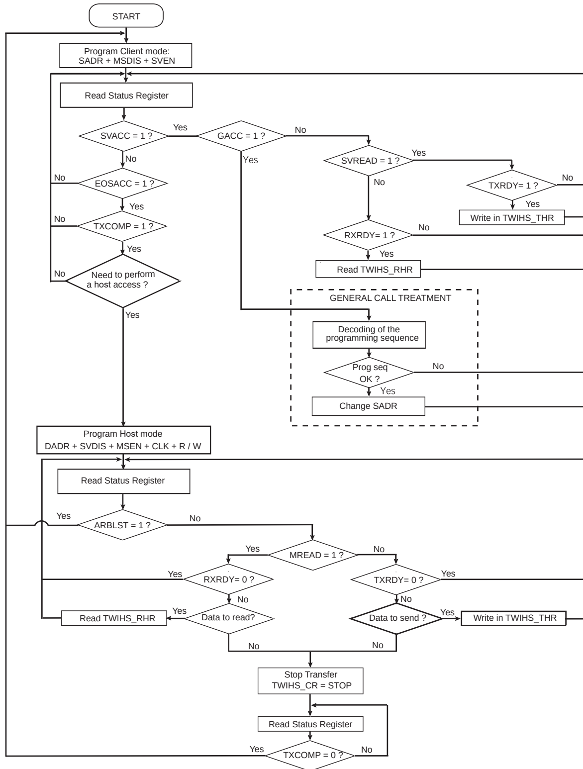
Figure 42-30. Multihost Flowchart
