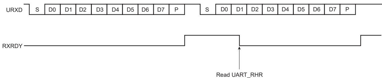
Figure 46-5. Receiver Ready
