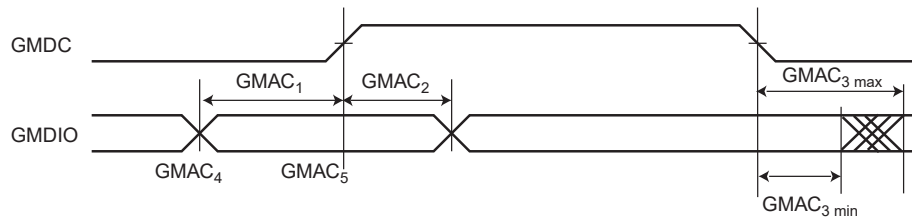
Figure 58-28. Min and Max Access Time of GMAC Output Signals
