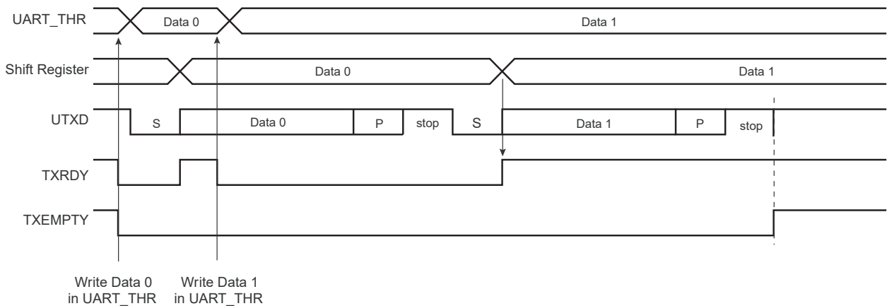
Figure 46-10. Transmitter Control
