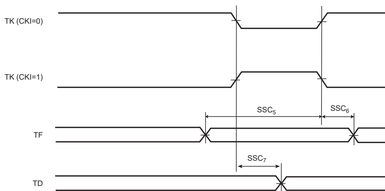
Figure 57-36. SSC Transmitter, TK and TF in Input
