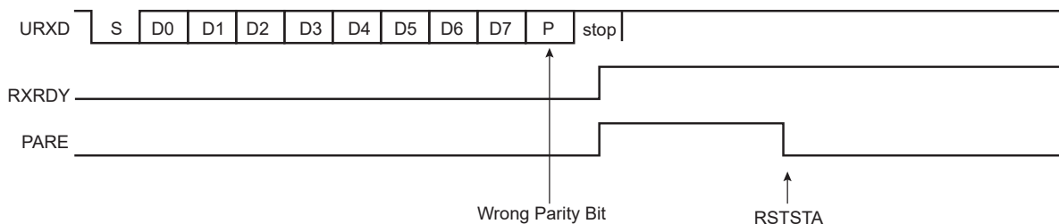
Figure 46-7. Parity Error
