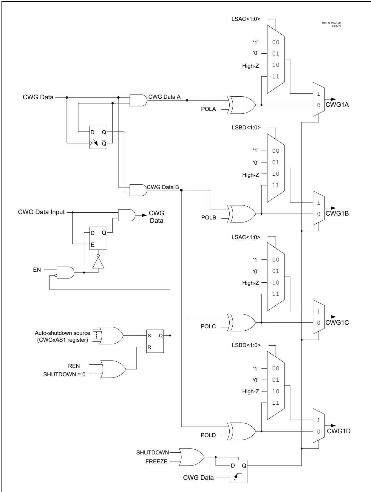
FIGURE 26-3: SIMPLIFIED CWG BLOCK DIAGRAM (PUSH PULL MODE, MODE[2:0] = 101)
