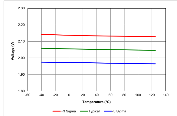
FIGURE 45-82: LPBOR Reset Voltage.
