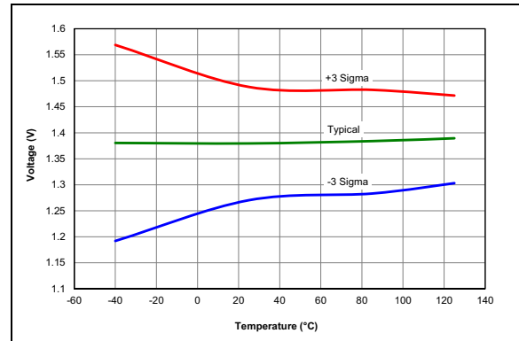
FIGURE 45-144: POR Release Voltage.
