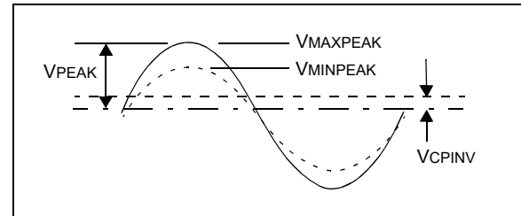
FIGURE 29-1: EXTERNAL VOLTAGE
