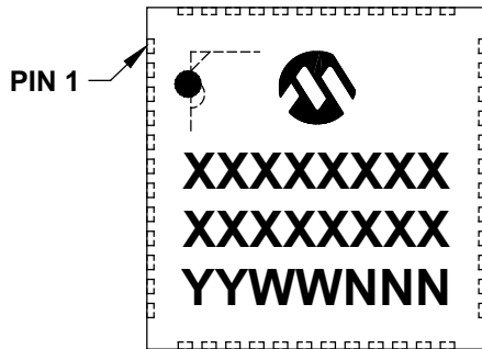
48-Lead VQFN (6x6x0.85 mm)
