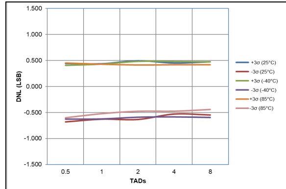
FIGURE 45-100: ADC 12-bit Mode, Single-Ended DNL, V_{DD} = 3.0V , V_{REF} = 3.0V , All devices.
