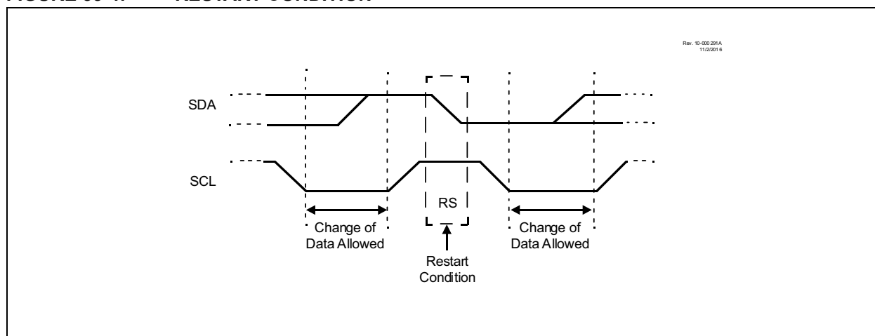
FIGURE 33-4: RESTART CONDITION
