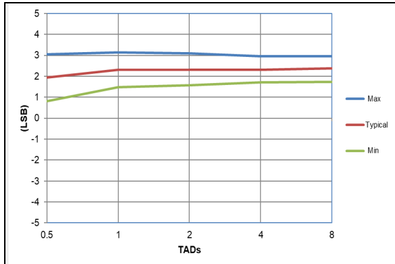
FIGURE 45-103: ADC 12-bit Mode, Single-Ended Offset, Error, V_{DD} = 3.0V , V_{REF} = 3.0V , -40°C to 85°C, All devices.
