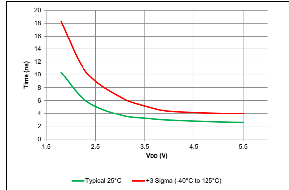
FIGURE 45-142: Fall Time, Slew Rate Control Disabled.
