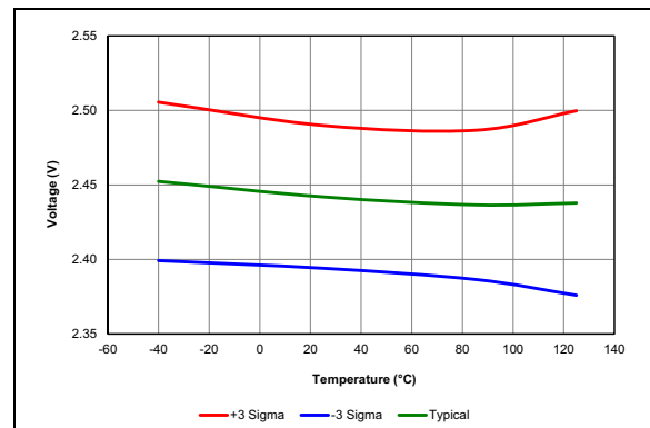
FIGURE 45-78: Brown-Out Reset Voltage, Trip Point (BORV = 10).
