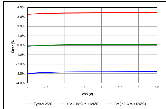
FIGURE 45-59: Calibrated HFINTOSC, Typical Frequency Error, PIC18F26/27/45/46/47/55/56/57K42 only.
