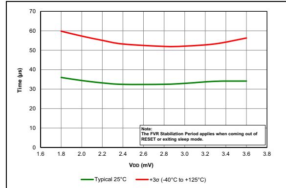
FIGURE 45-130: FVR Stabilization Period, PIC18LF26/27/45/46/47/55/56/57K42 Only.
