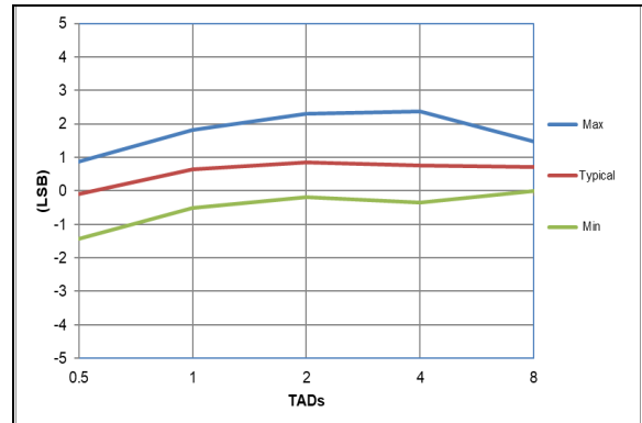
FIGURE 45-102: ADC 12-bit Mode, Single-Ended Gain, Error, V_{DD} = 3.0V , V_{REF} = 3.0V , -40°C to 85°C, All devices.
