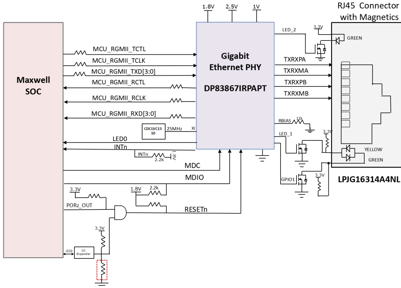
Figure 4-15. MCU Gigabit Ethernet Block
