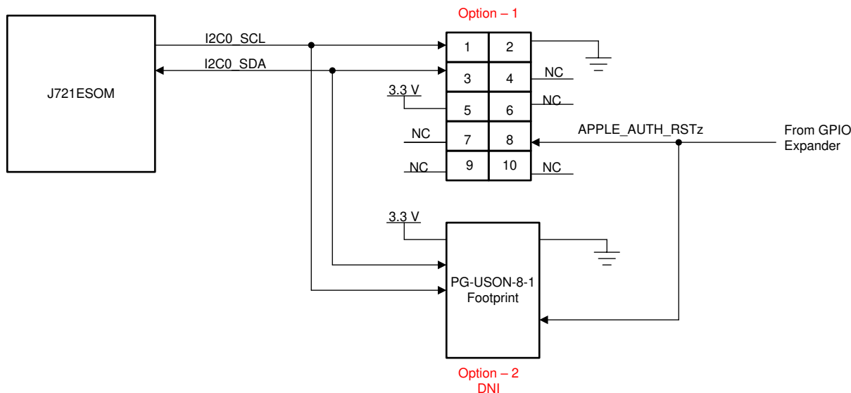
Figure 4-42. Apple Authentication Block Diagram
