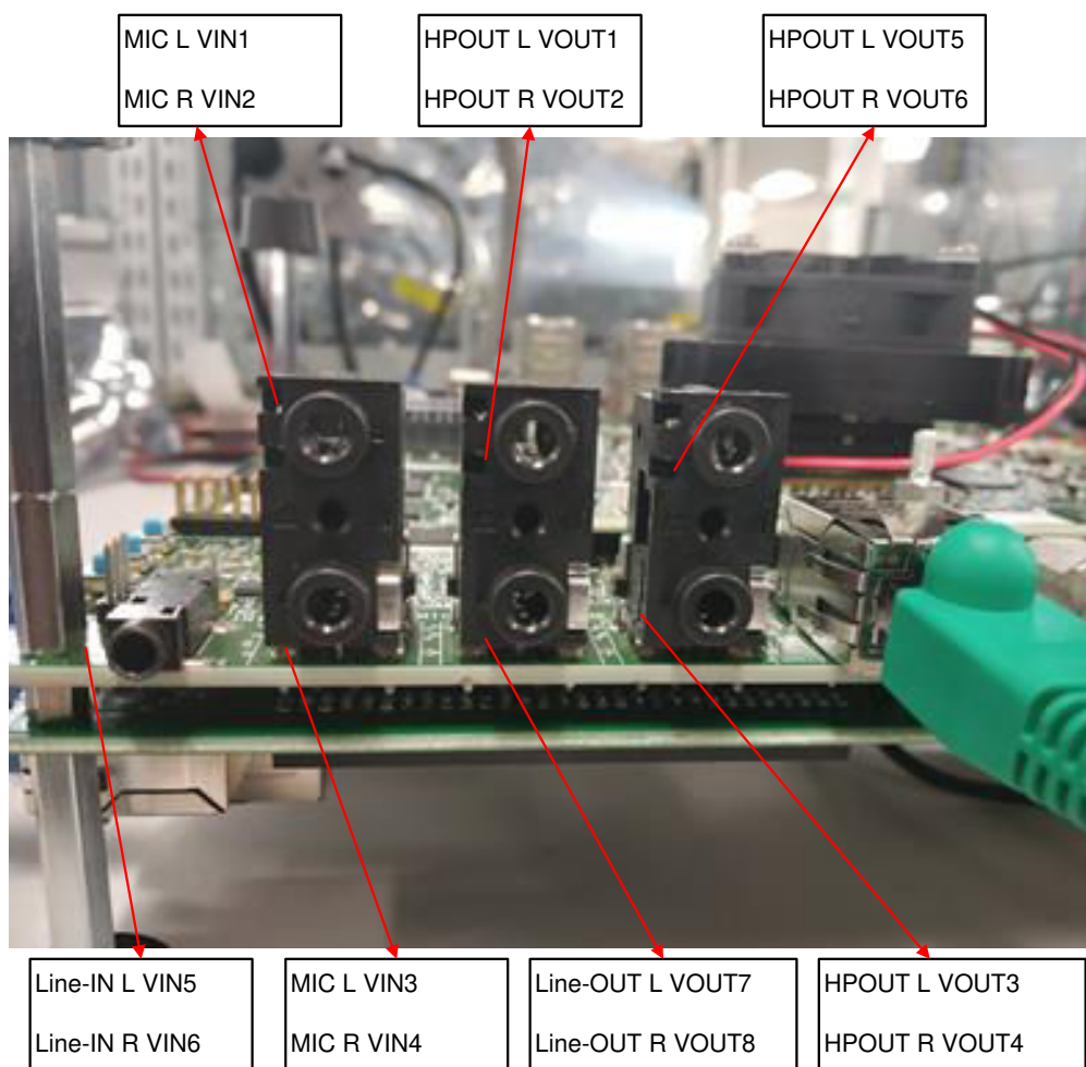
Figure 4-37. Audio Port Interface Assignment
