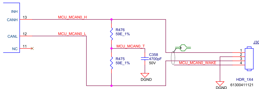
Figure 4-31. MCU CAN0 Interface
