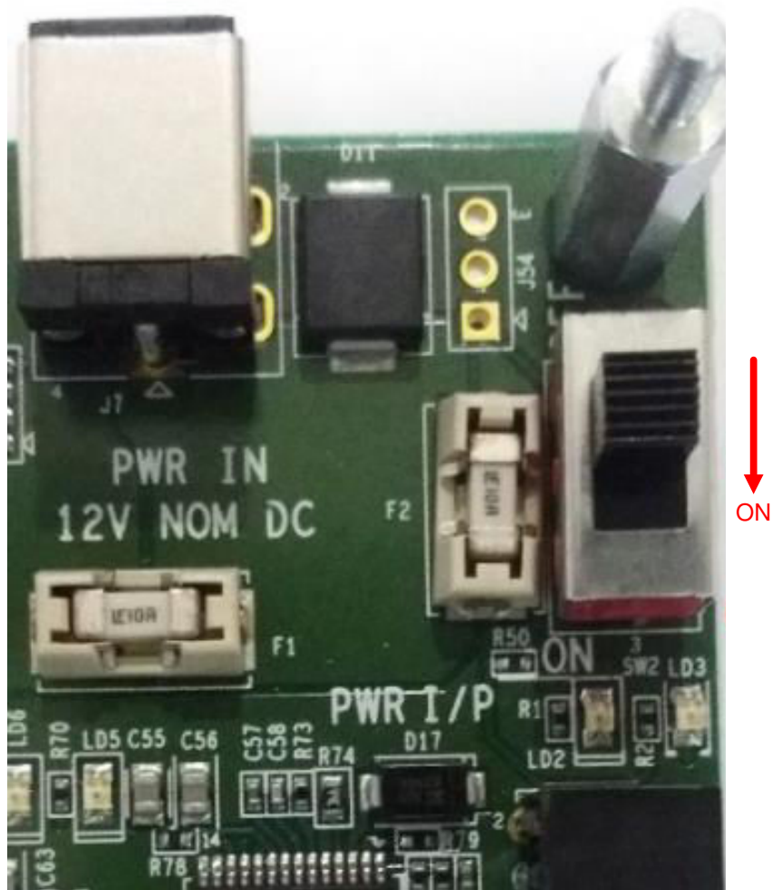
Figure 3-2. Power ON/OFF Switch
