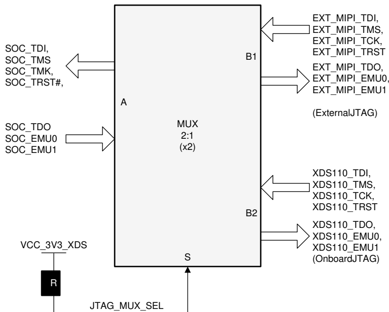
Figure 3-8. JTAG Mux
