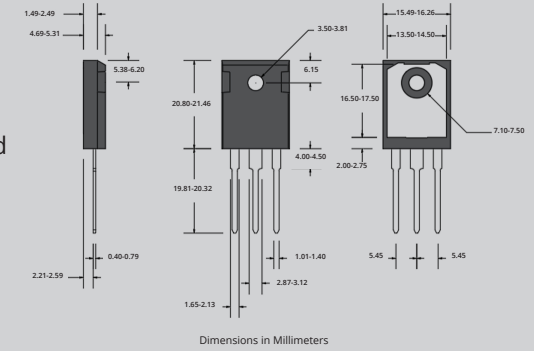
TO-247-3-Lead
