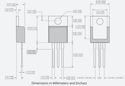
TO-220 3-Lead
