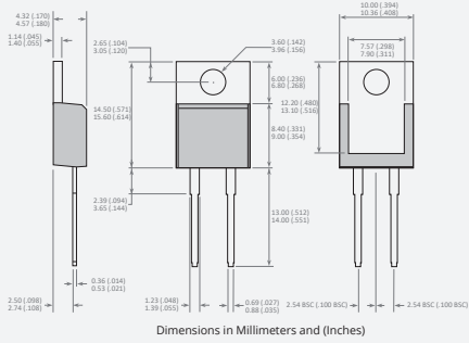
TO-220 2-Lead
