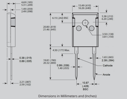
TO-247 2-Lead
