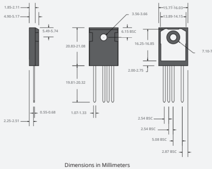
TO-247-4-Lead
