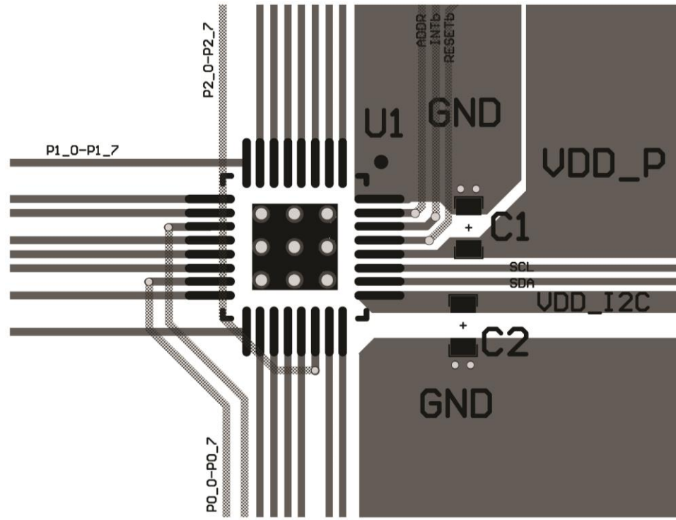
Figure 7. Recommended Layouts for TQFN55-32
