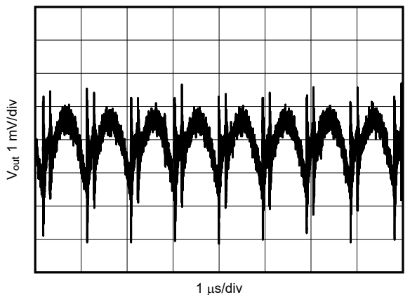
12 V to 1.8 V, 1 A 2.2 \mu\text{H} , 1 MHz First L-C Only Figure 6-5. V_{OUT} Ripple After the First L-C Filter
