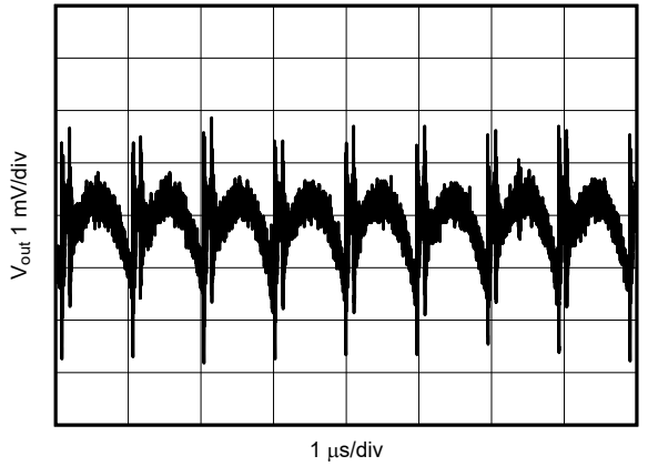
12 V to 1.2 V, 1 A 2.2 \mu\text{H} , 1 MHz First L-C Only Figure 6-1. V_{OUT} Ripple After the First L-C Filter
