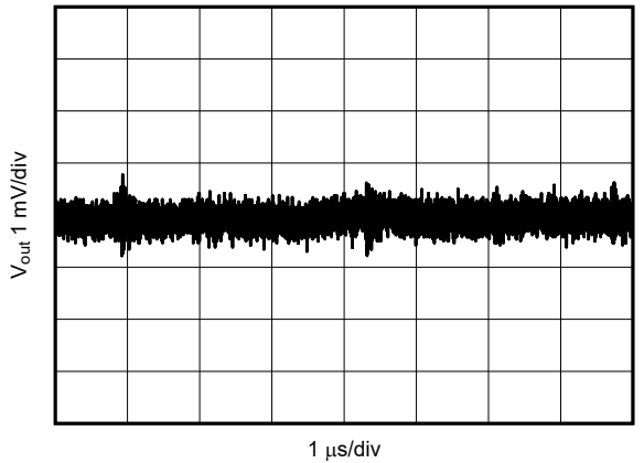
12 V to 1.2 V, 1 A 2.2 \mu\text{H} , 1 MHz First and second L-C Figure 6-3. V_{OUT} Ripple After the Second L-C Filter
