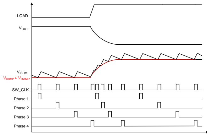
Figure 10. Load Insertion
