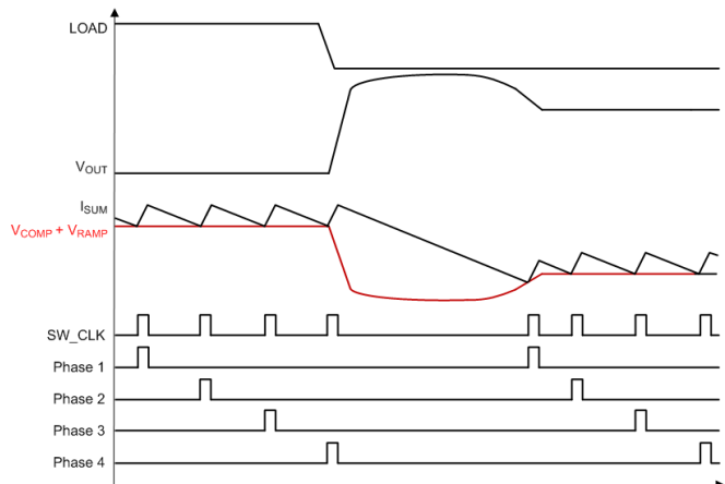
Figure 11. Load Release
