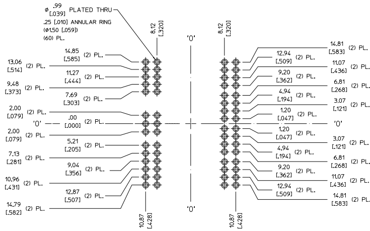
RECOMMENDED LAND PATTERN (COMPONENT SIDE SHOWN)
