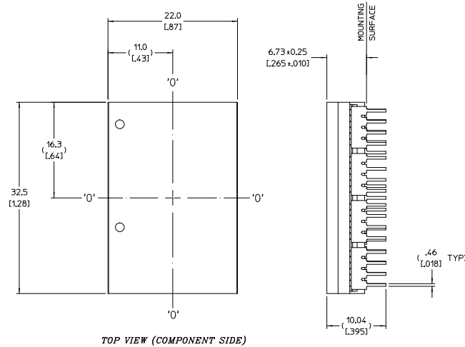
TOP VIEW (COMPONENT SIDE)
