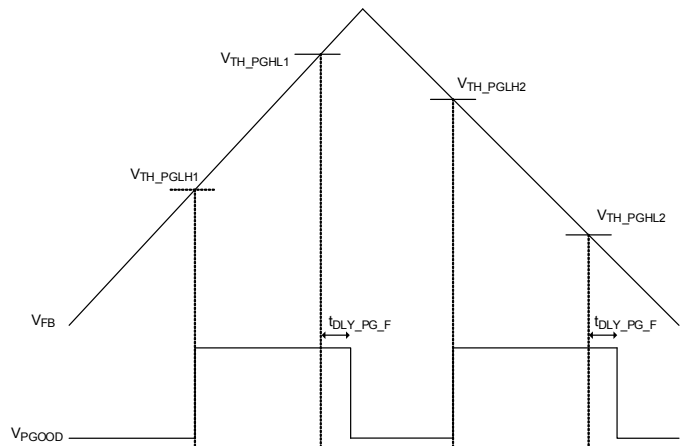
Figure 4. The Logic of PGOOD
