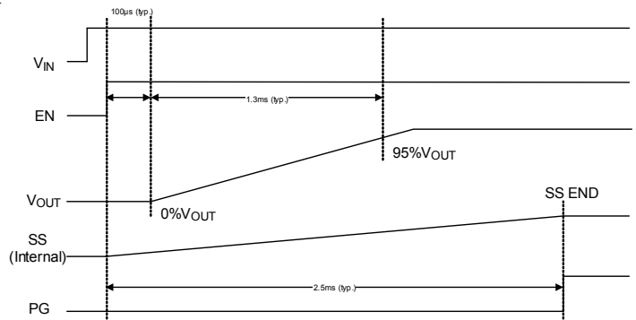
Figure 3. Start-Up Sequence
