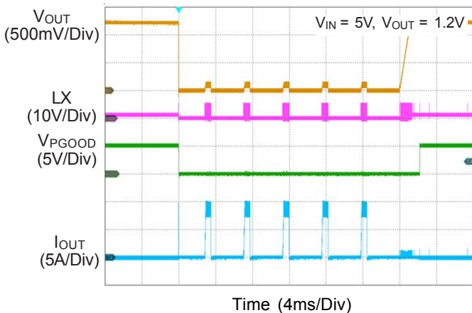
Figure 2. Short-Circuit Protection and Recovery
