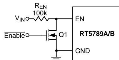
Figure 6. Logic Control for the EN Pin
