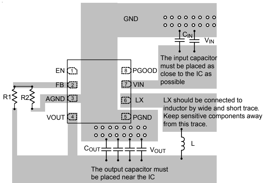
Figure 10. UDFN-8L 2.5x2 (FC) PCB Layout Guide
