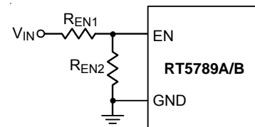
Figure 7. Resistor Divider for Under-Voltage Lockout Threshold Setting
