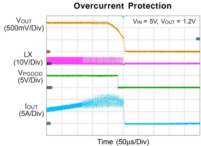
Figure 1. Overcurrent Protection
