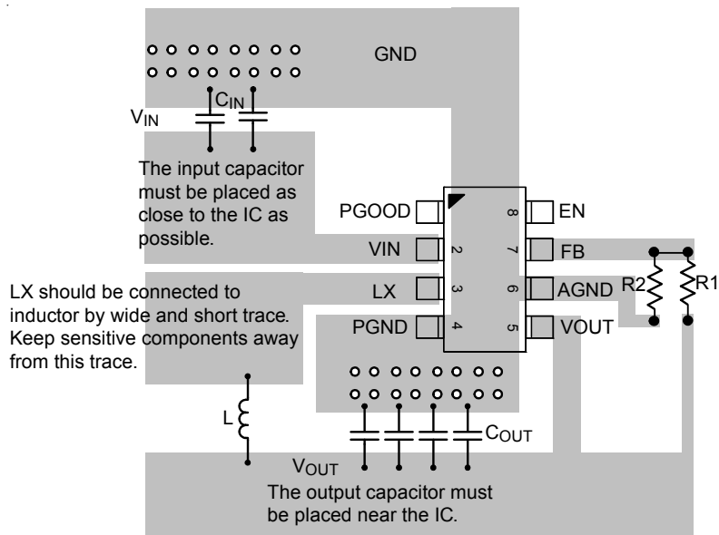
Figure 10. TSOT-23-8 (FC) PCB Layout Guide
