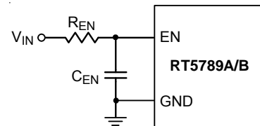
Figure 5. Enable Timing Control
