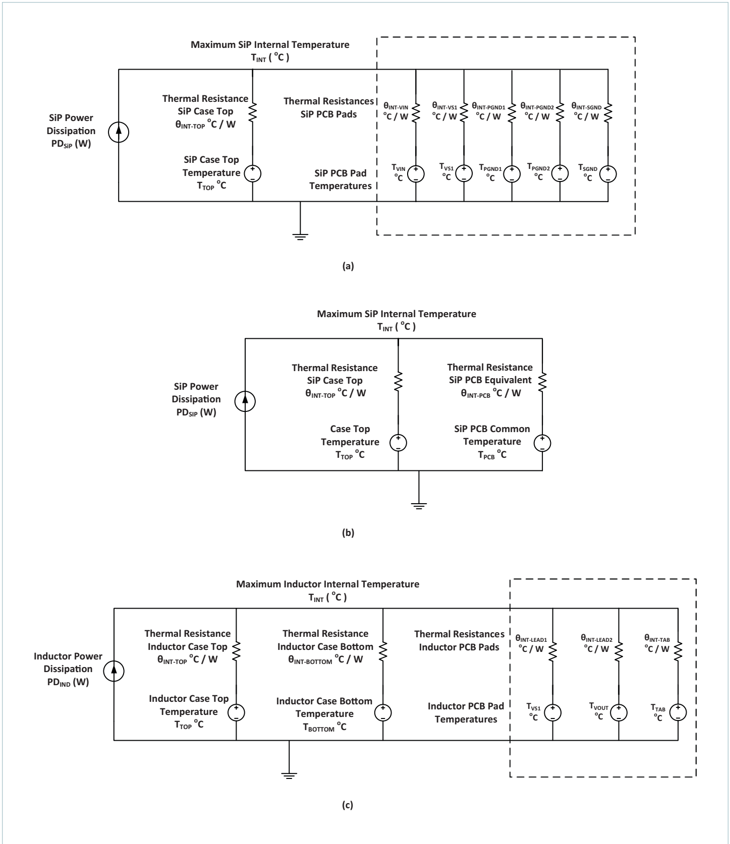
Figure 59 — PI3325-00 thermal model (a), SiP simplified version (b) and inductor thermal model (c)
