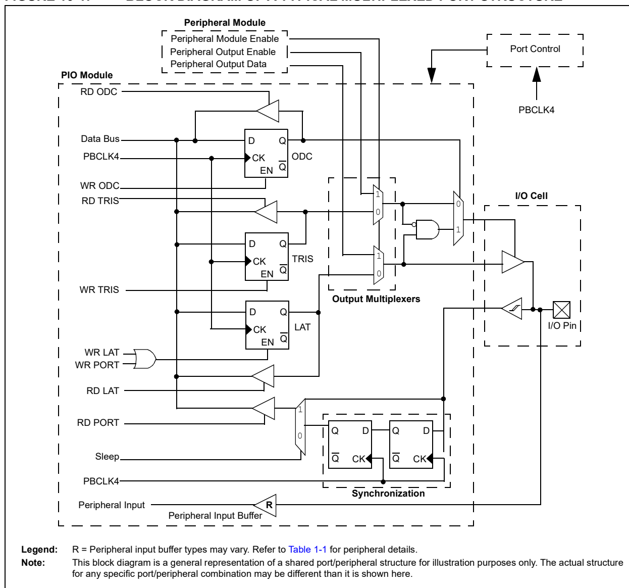
FIGURE 10-1: BLOCK DIAGRAM OF A TYPICAL MULTIPLEXED PORT STRUCTURE
