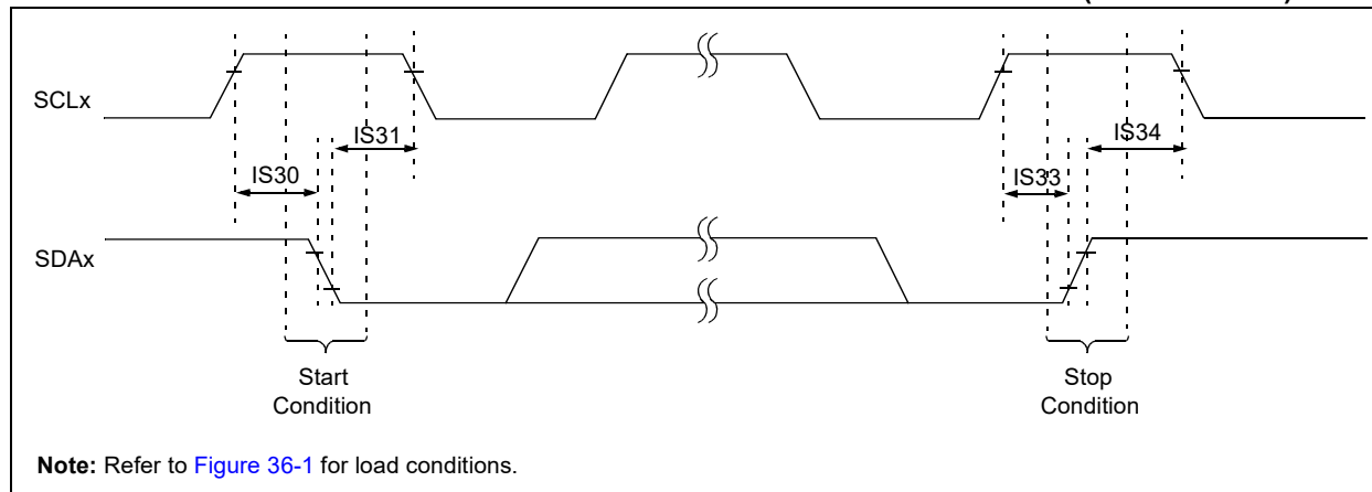
FIGURE 36-16: I2Cx BUS START/STOP BITS TIMING CHARACTERISTICS (SLAVE MODE)
