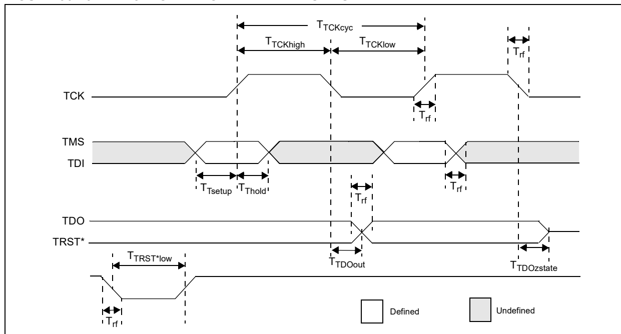
FIGURE 36-23: EJTAG TIMING CHARACTERISTICS
