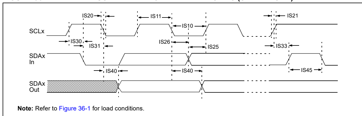
FIGURE 36-17: I2Cx BUS DATA TIMING CHARACTERISTICS (SLAVE MODE)
