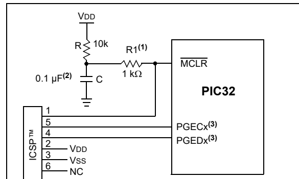
FIGURE 2-2: EXAMPLE OF MCLR PIN CONNECTIONS
