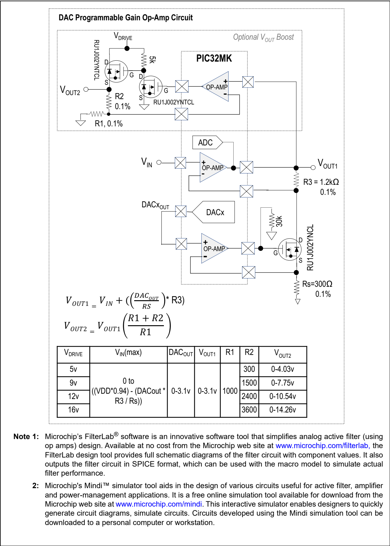
FIGURE 25-18: OP AMP CONFIGURATION CIRCUIT EXAMPLES
