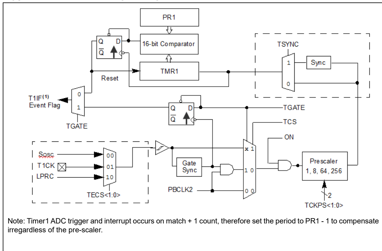
FIGURE 11-1: TIMER1 BLOCK DIAGRAM
