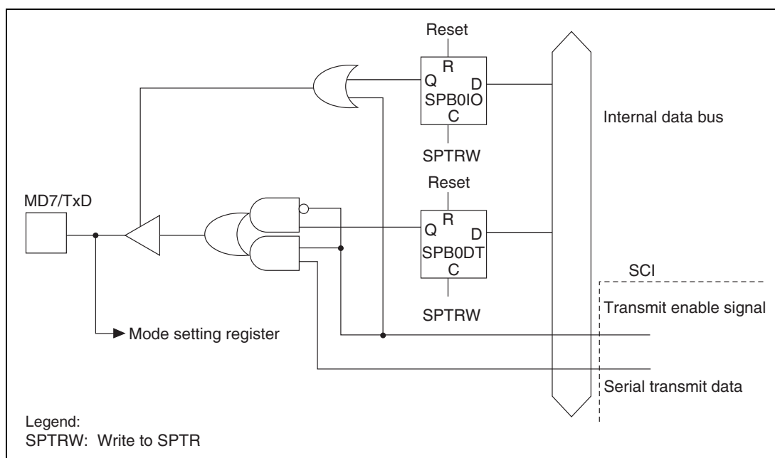
Figure 15.3 MD7/TxD Pin
