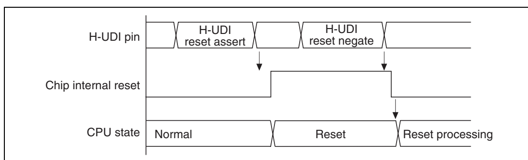
Figure 21.3 H-UDI Reset
