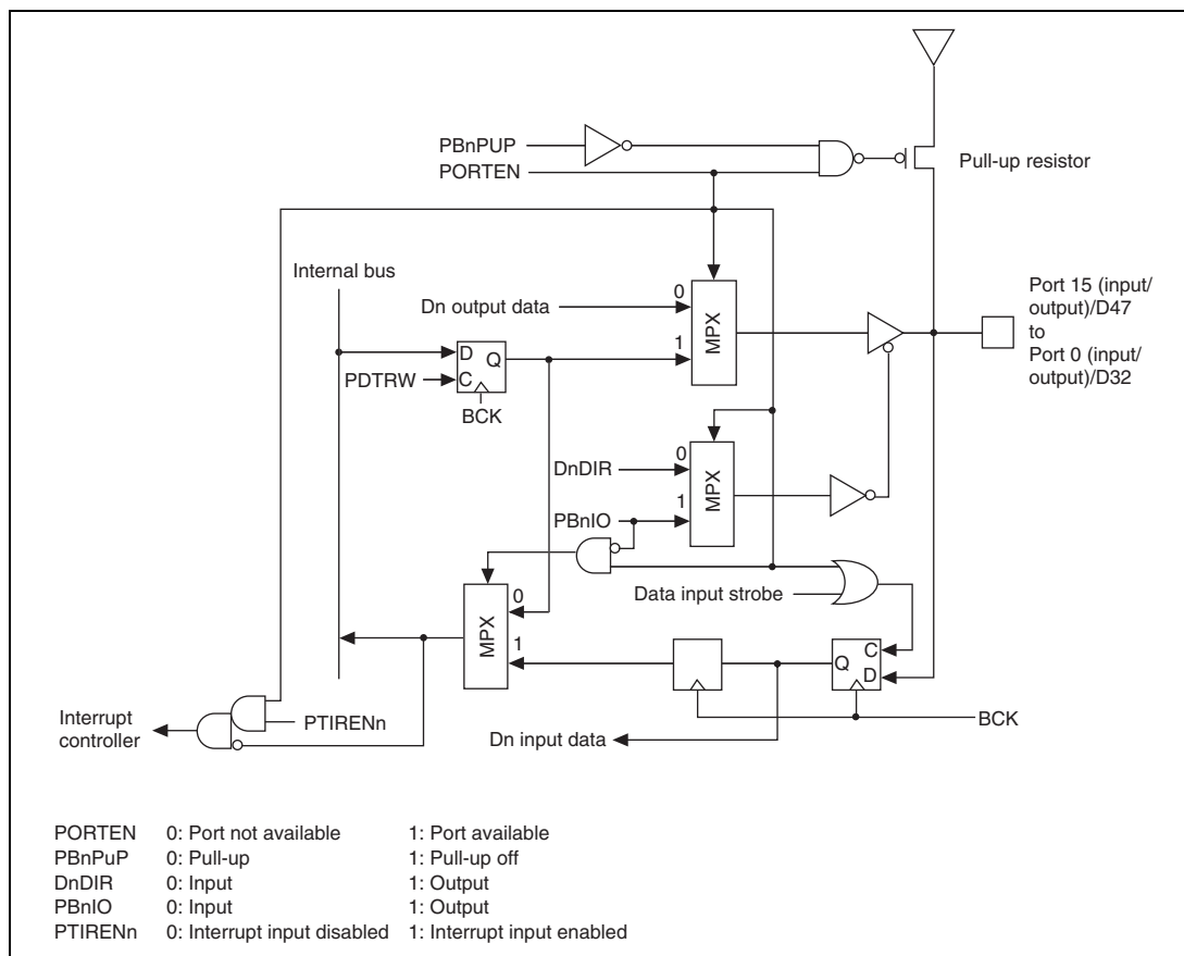
Figure 18.1 16-Bit Port
