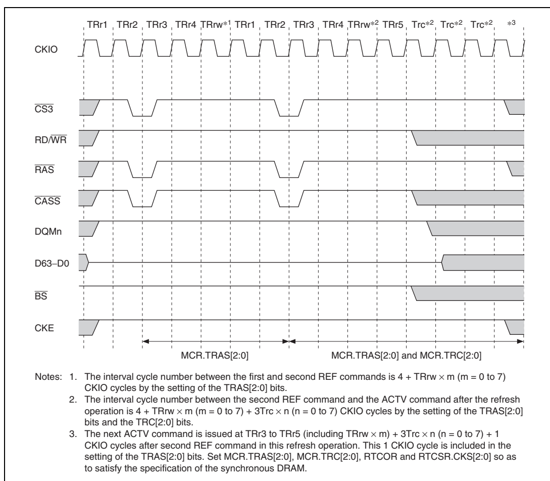
Figure 13.46 Synchronous DRAM Auto-Refresh Timing with 64-Bit Bus Width ( \text{TRAS}[2:0] = 001 , \text{TRC}[2:0] = 001 )
