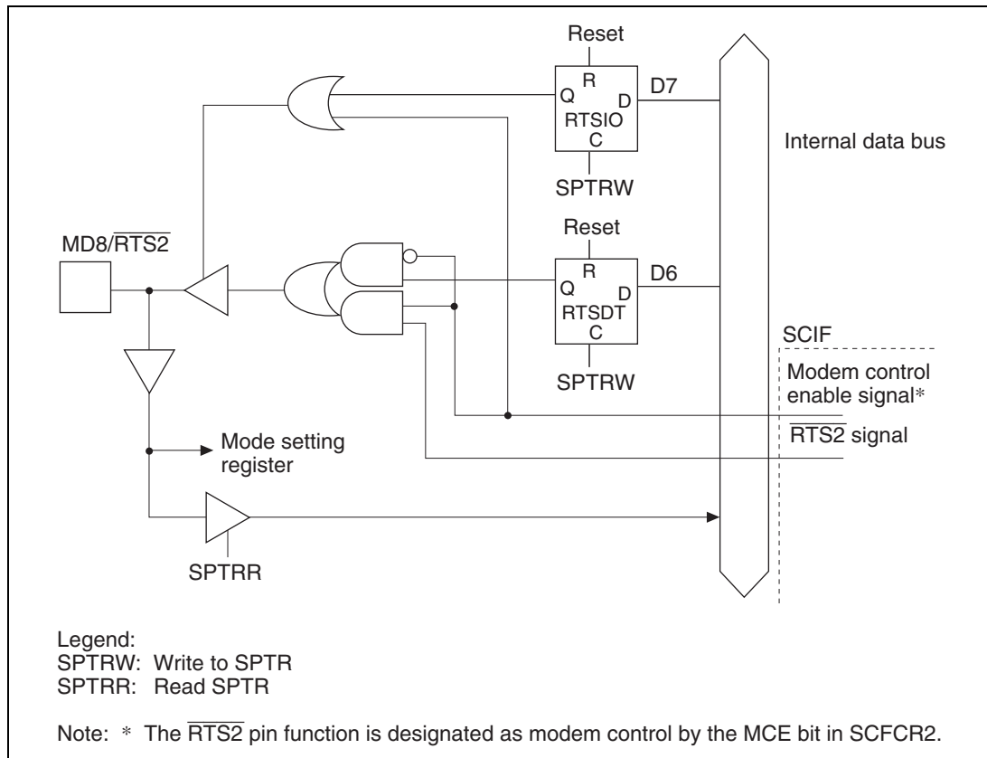
Figure 16.2 MD8/RTS2 Pin
