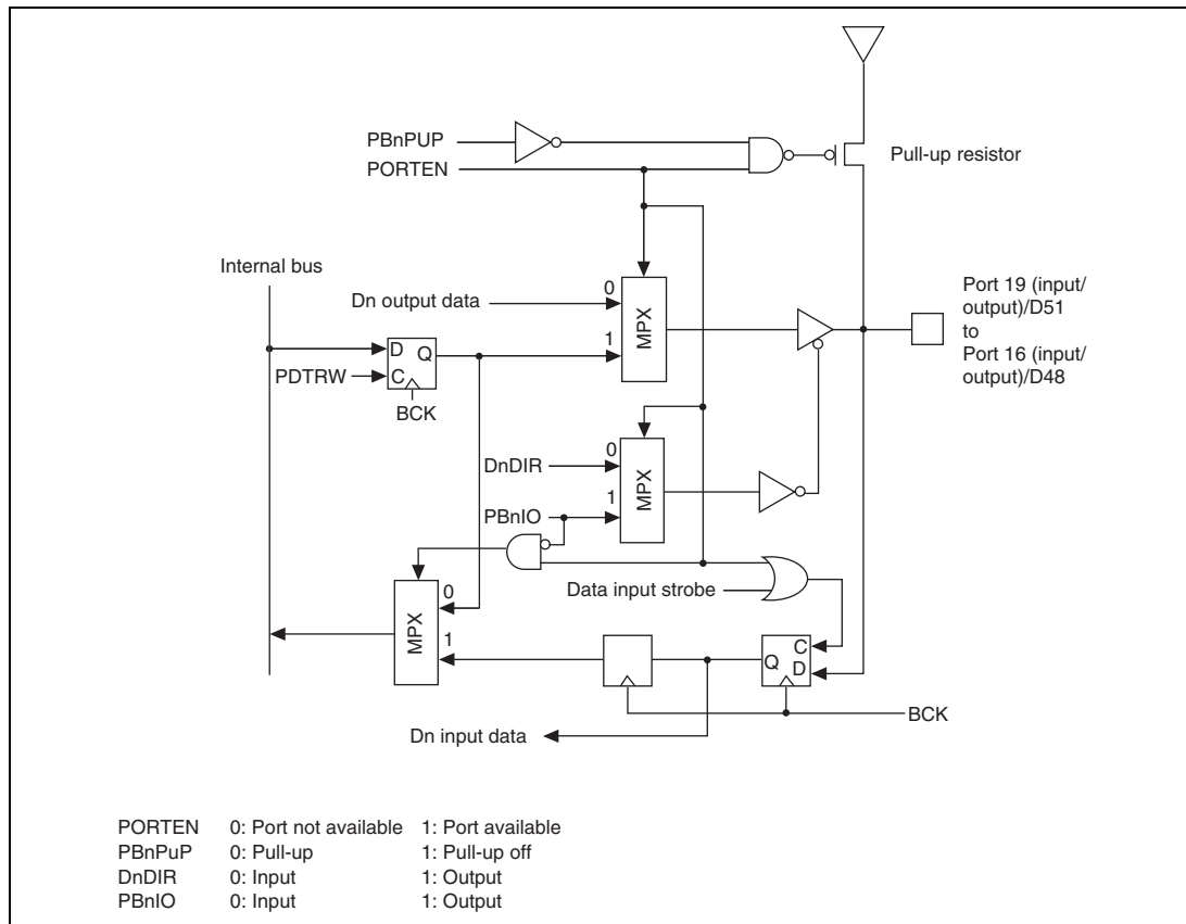
Figure 18.2 4-Bit Port
