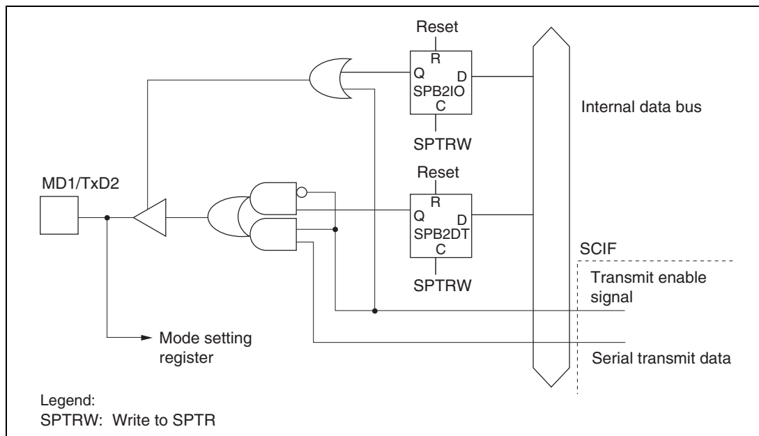
Figure 18.6 MD1/TxD2 Pin
