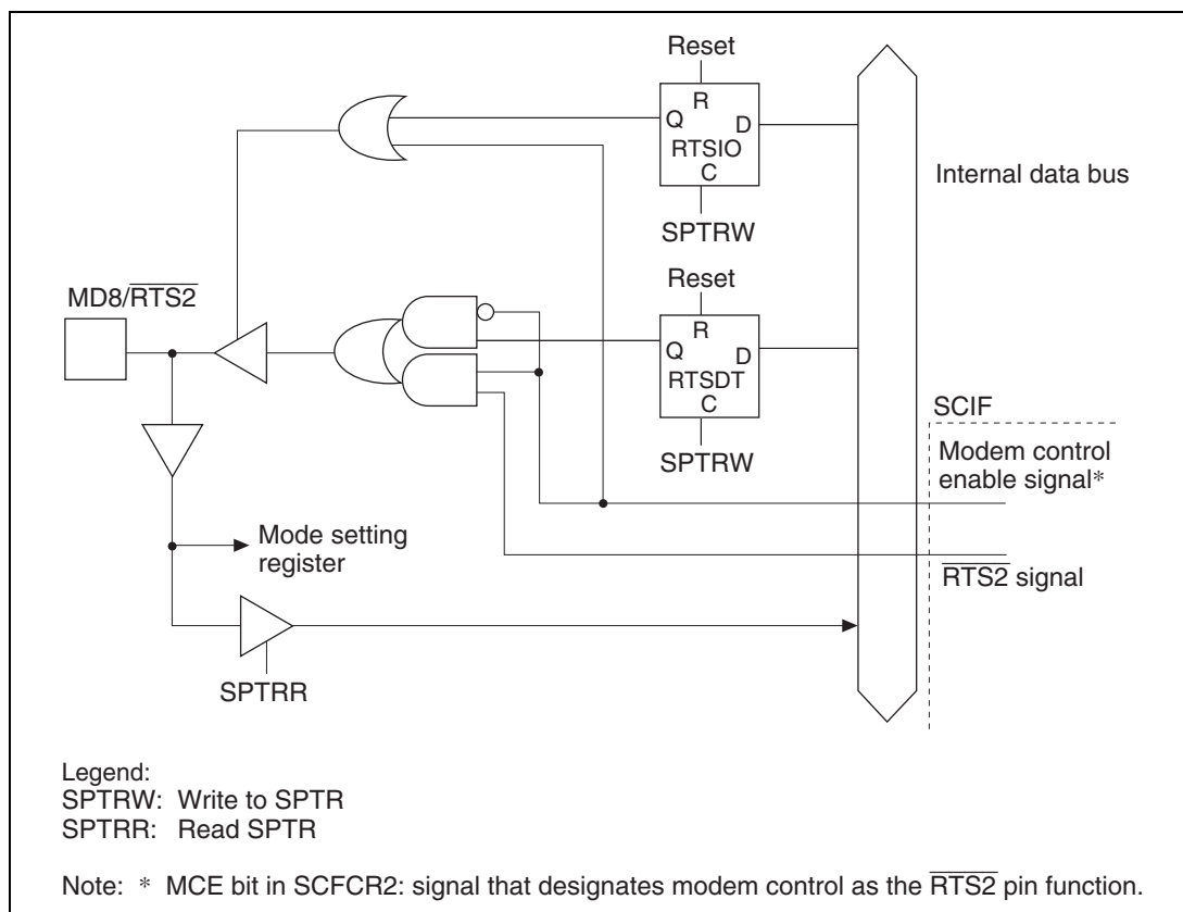
Figure 18.9 MD8/RTS2 Pin
