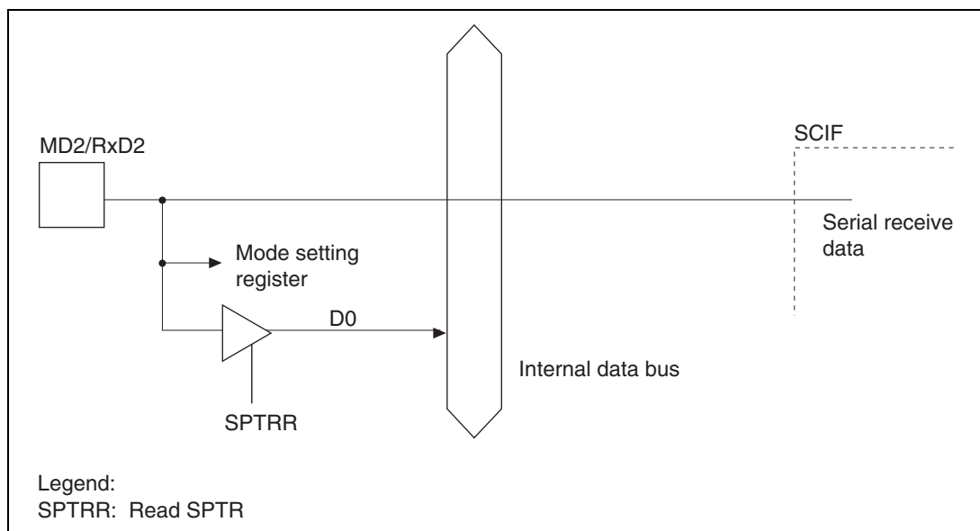
Figure 16.5 MD2/RxD2 Pin
