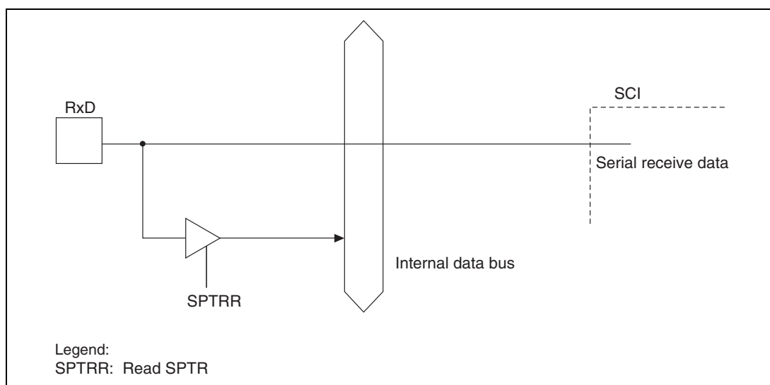
Figure 15.4 RxD Pin
