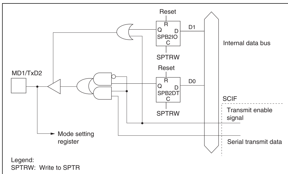
Figure 16.4 MD1/TxD2 Pin
