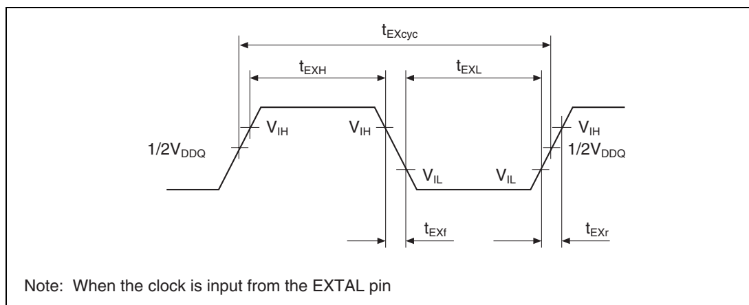
Figure 22.1 EXTERNAL Clock Input Timing
