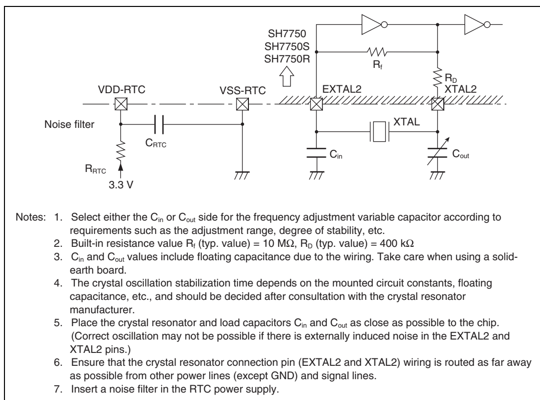
Figure 11.5 Example of Crystal Oscillator Circuit Connection
