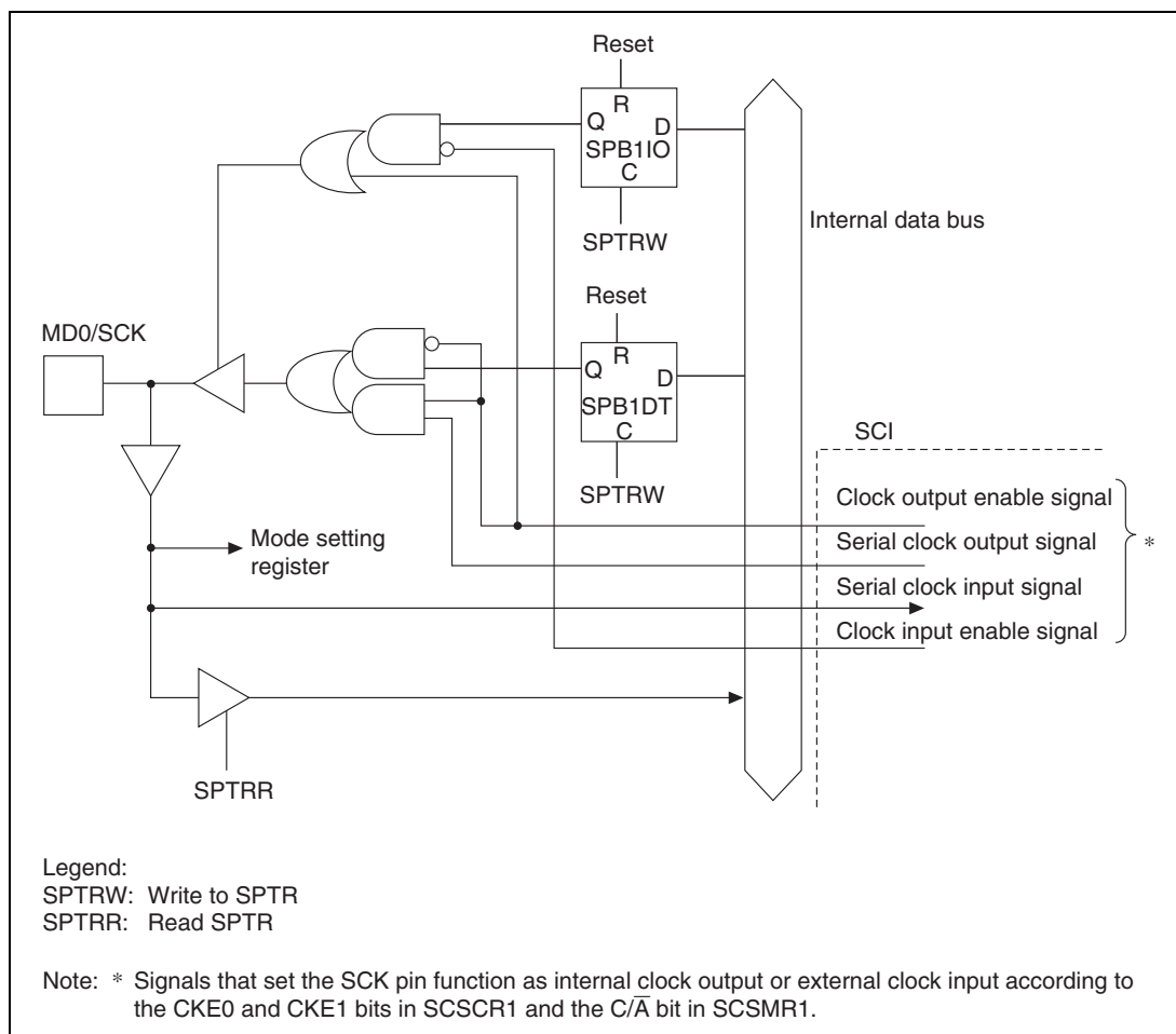
Figure 18.3 MD0/SCK Pin
