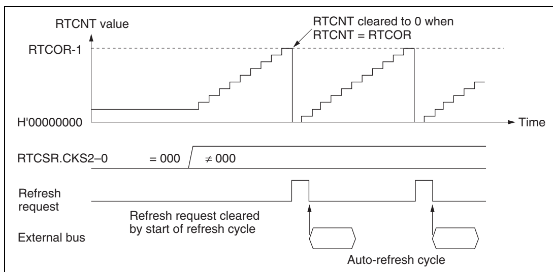
Figure 13.39 Auto-Refresh Operation
