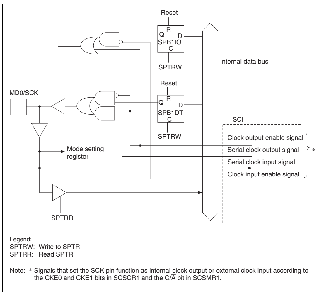
Figure 15.2 MD0/SCK Pin
