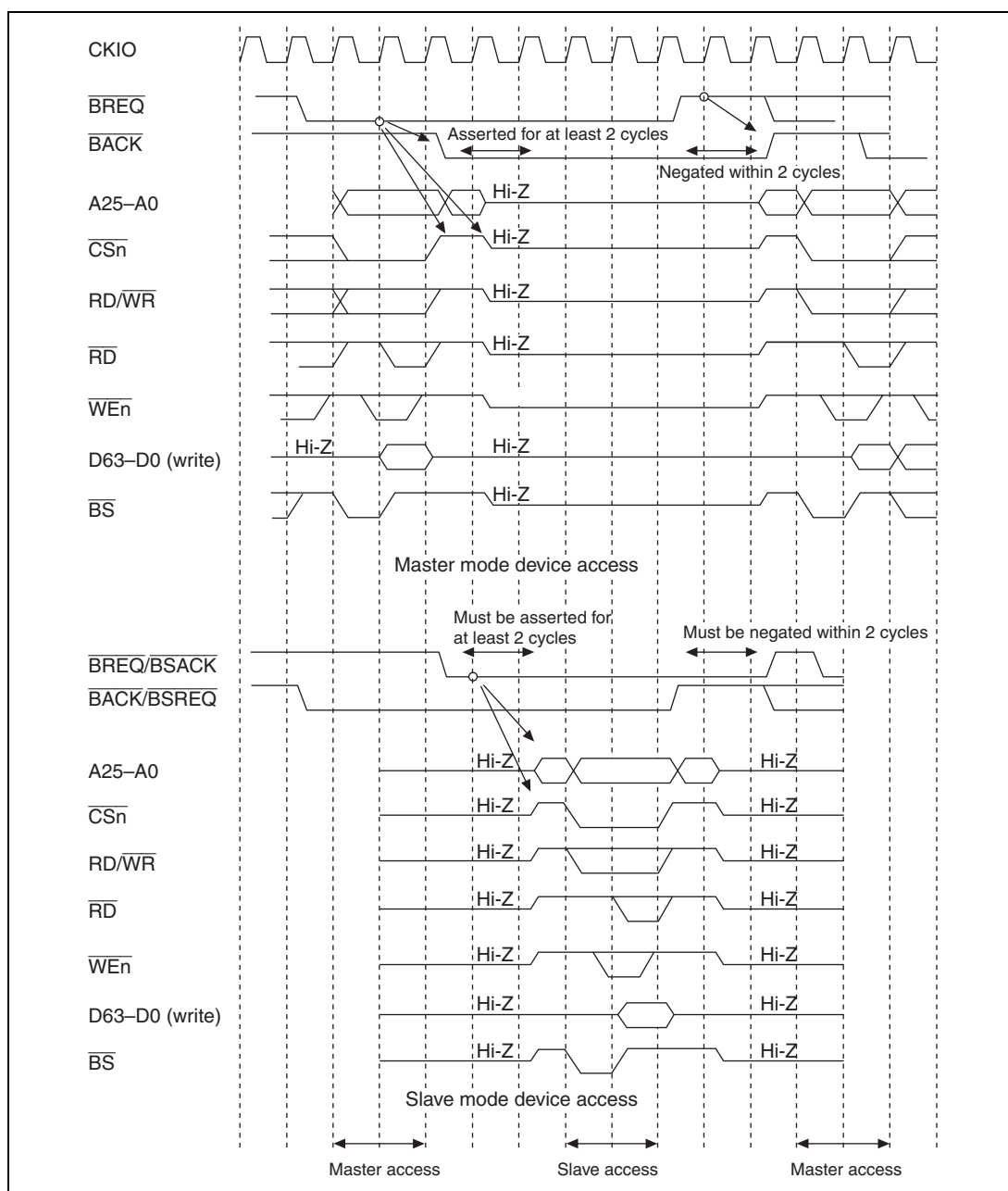
Figure 13.79 Arbitration Sequence
