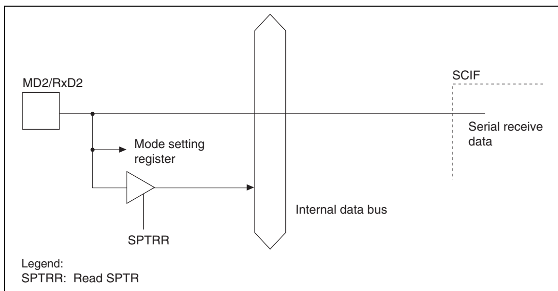
Figure 18.7 MD2/RxD2 Pin
