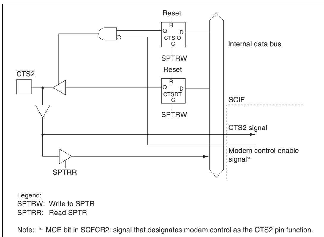
Figure 18.8 \overline{\text{CTS2}} Pin
