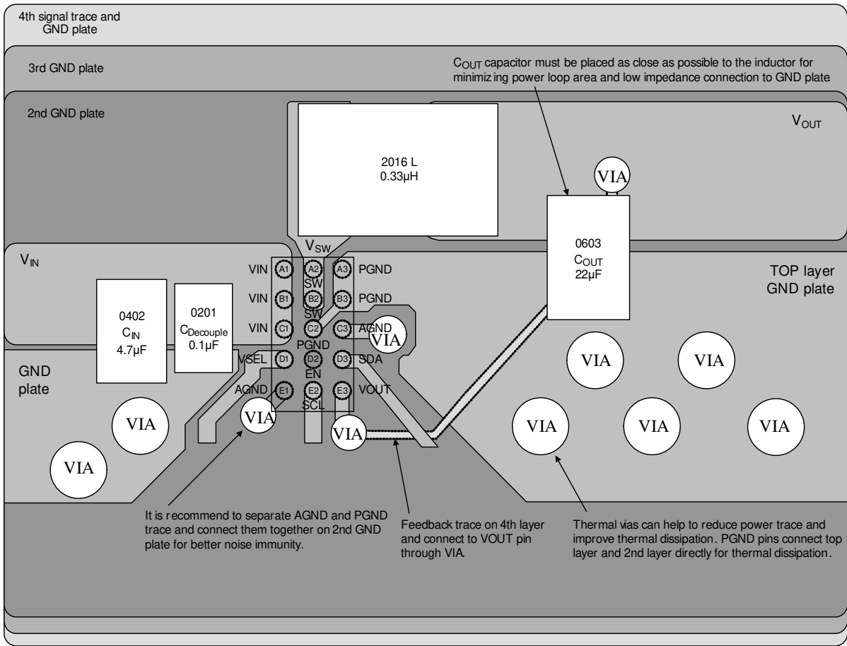
Figure 4-5. PCB layout guide
