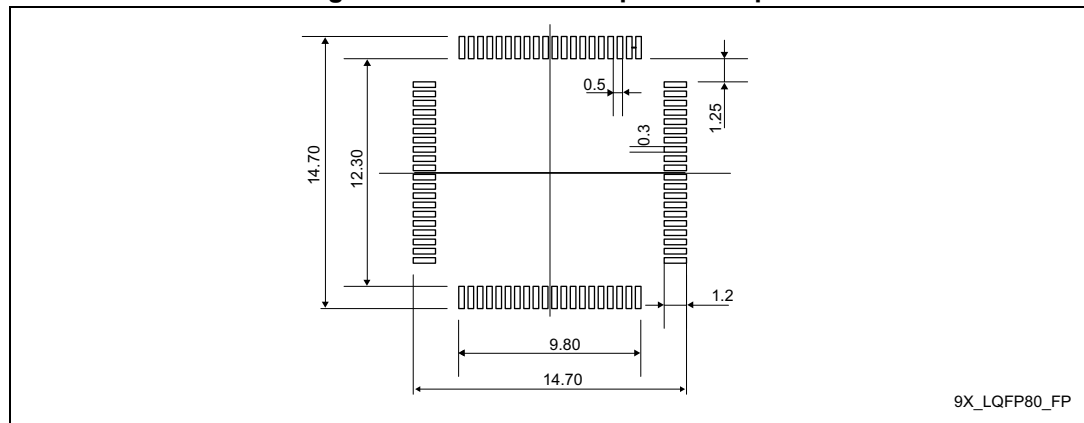
Figure 56. LQFP80 - Footprint example
