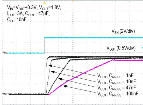
Time (4ms/div)
