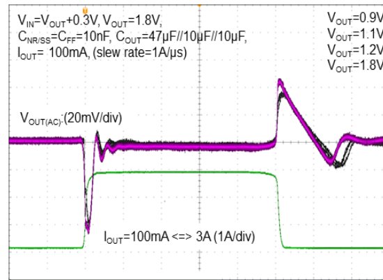
Time (20μs/div)
