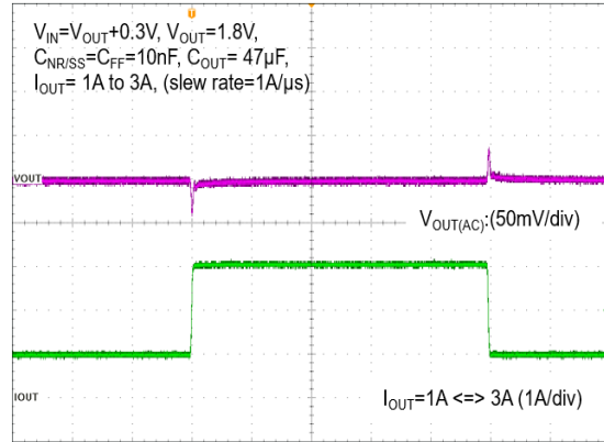
Time (100μs/div)
