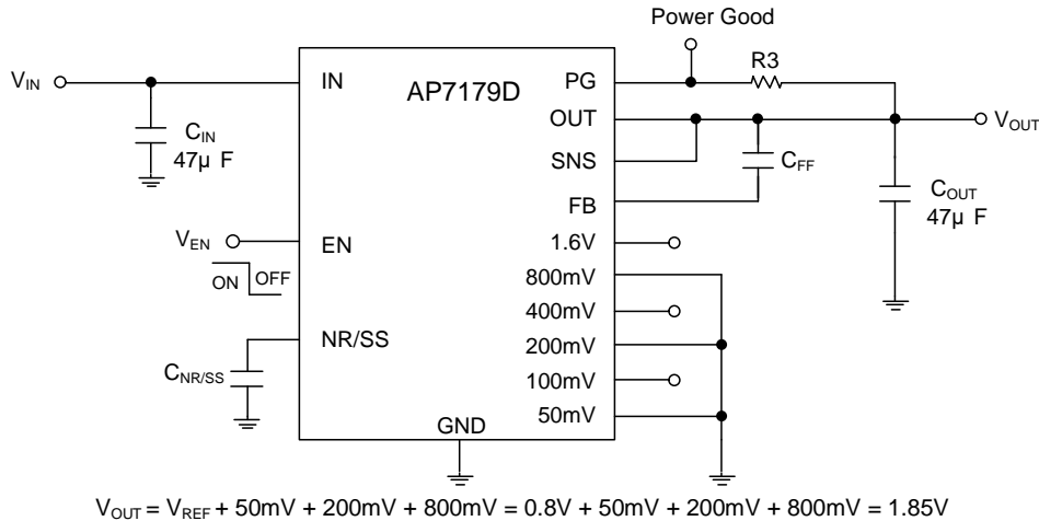
Figure 4. Output voltage set by programming pins
