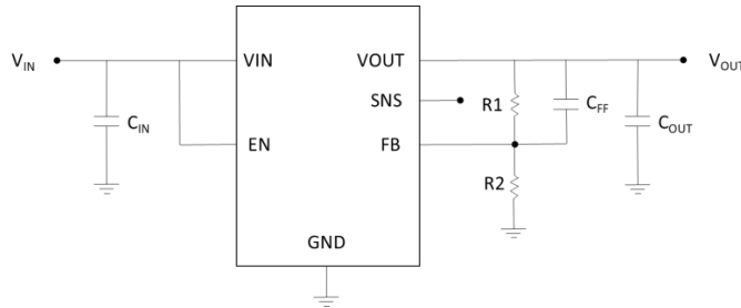
Figure 3. Output voltage set by external resistors
