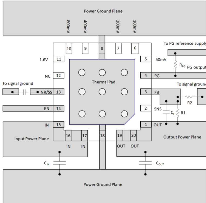
Figure 6. PCB Layout Guide
