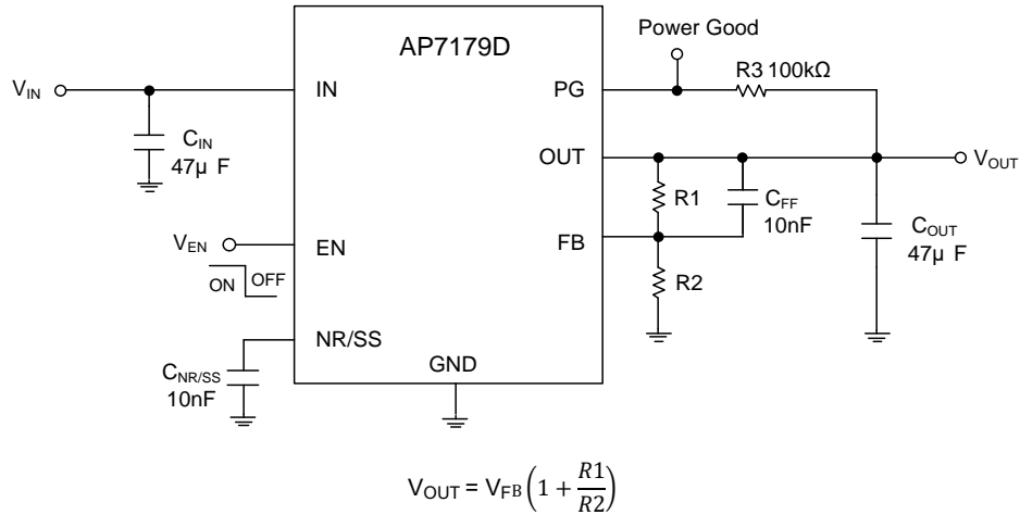
Figure 1. Configuration Circuit for V OUT Adjusted by a Resistive Divider
