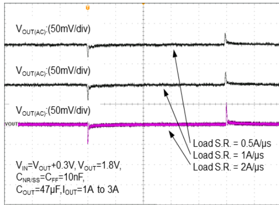
Time (100μs/div)
