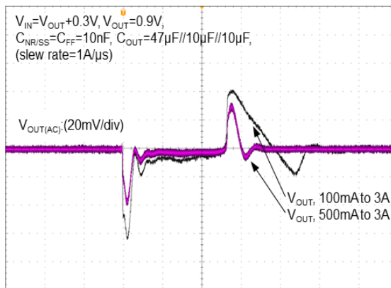
Time (20μs/div)
