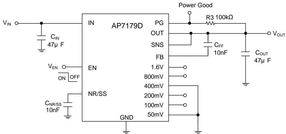
Figure 2. Configuration Circuit for V OUT Adjusted via PCB layout
