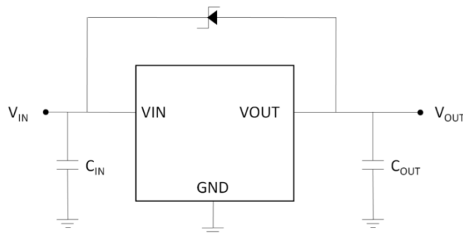
Figure 5. Application circuit for reverse current protection
