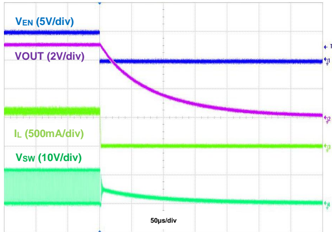
Figure 21. Shutdown Using EN, IOOUT = 600mA
