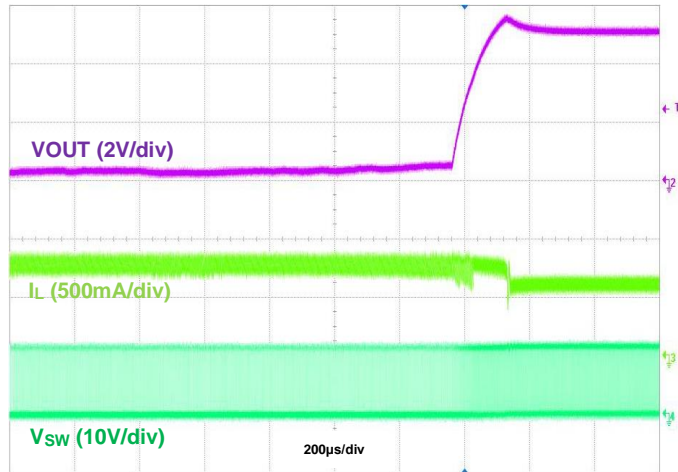
Figure 23. Output Short Recovery, IOOUT = 600mA
