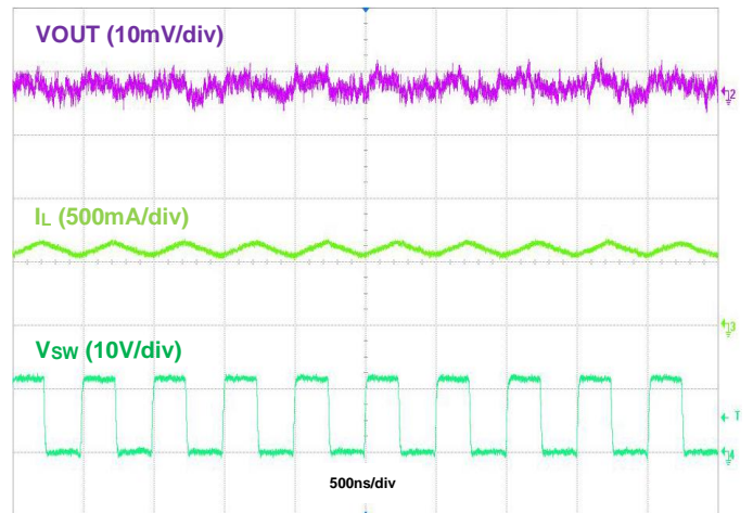
Figure 15. Output Voltage Ripple, VOUT = 5V; IOUT = 600mA
