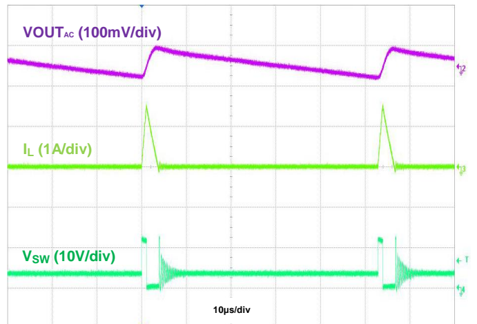
Figure 22. Output Ripple, VIN=12V, VOUT = 3.3V @50mA, PFM
