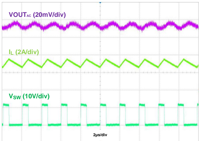
Figure 21. Output Ripple, VIN=12V, VOUT = 3.3V @3A, PFM
