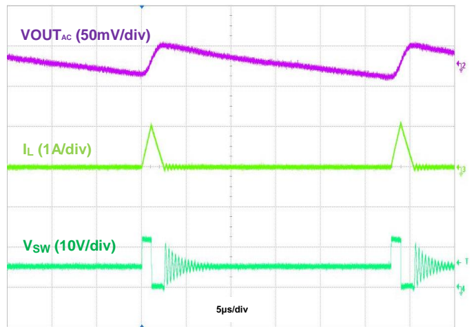
Figure 18. Output Ripple VIN = 12V, VOUT = 5V @50mA, PFM
