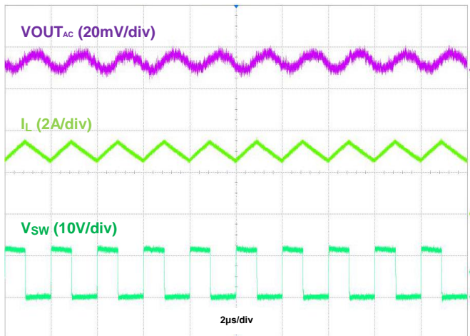
Figure 19. Output Ripple, VIN=12V, VOUT = 5V @3A, PWM
