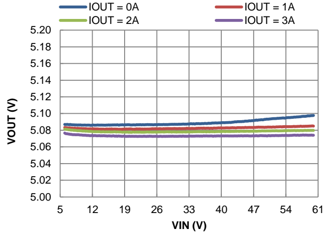
Figure 14. Line Regulation
