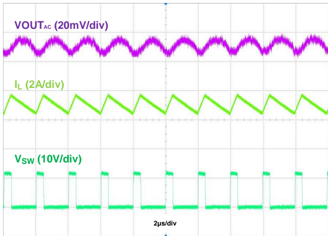
Figure 17. Output Ripple, VIN=12V, VOUT = 5V @3A, PFM
