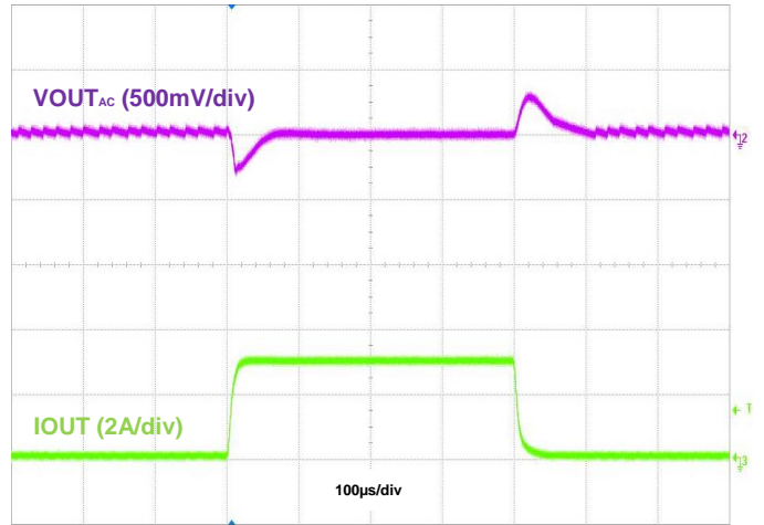
Figure 30. Load Transient, IOUT = 50mA to 3A to 50mA, PFM
