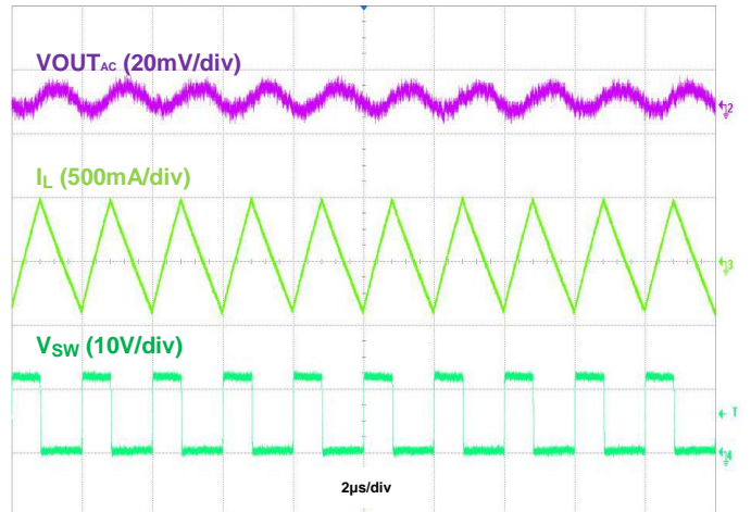
Figure 20. Output Ripple VIN = 12V, VOUT = 5V @50mA, PWM
