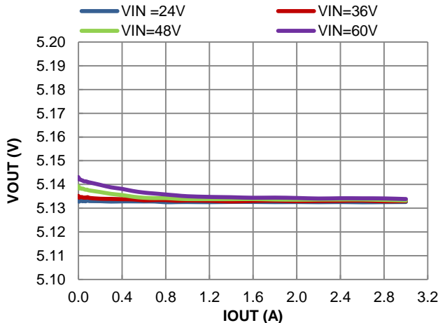
Figure 15. Load Regulation
