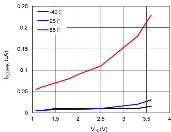
Leakage Current vs. Input voltage
