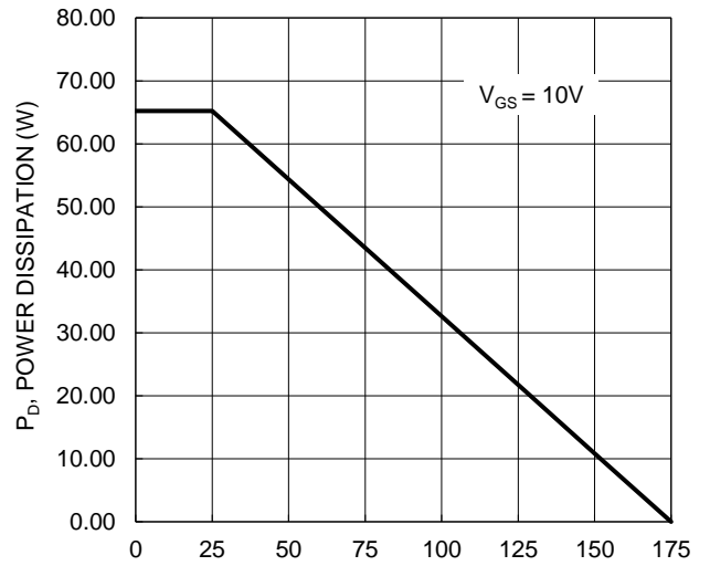
T C , CASE TEMPERATURE (°C) Figure 14. Power Dissipation Function of T C
