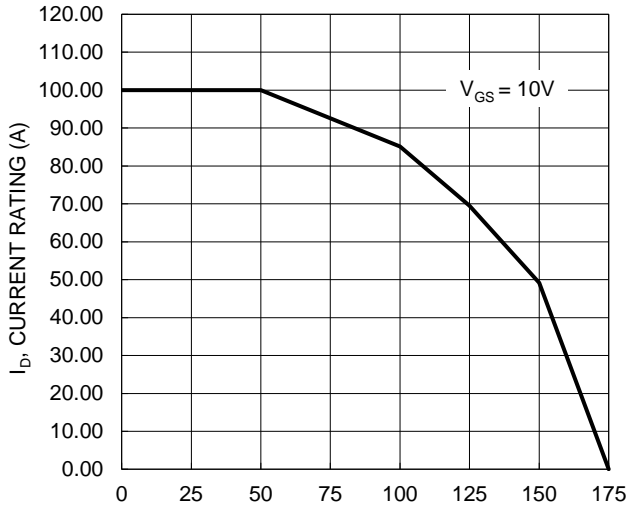
T C , CASE TEMPERATURE (°C) Figure 13. Current Function of T C
