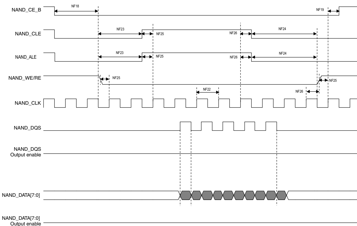
Figure 32. Source Synchronous Mode Data Read Timing Diagram
