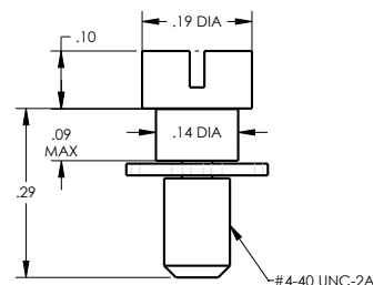
#4/40 M83513/05-13
