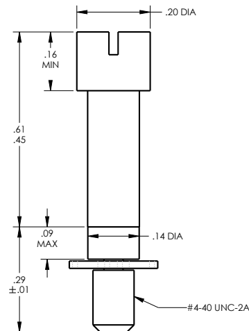
#4/40 M83513/05-16
