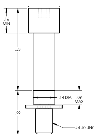
#4/40 M83513/05-15
