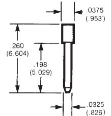
24 Gauge Stainless Steel Guide Pin*
