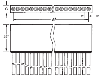
Pin Connector
