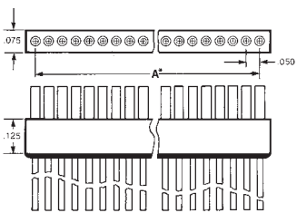
Socket Connector
