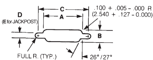
Figure 2: Rear Mounting
