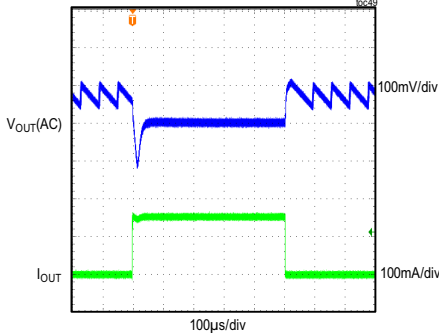
MAXM15065 LOAD TRANSIENT RESPONSE V_{IN} = 24V , FIXED V_{OUT} = 3.3V , PFM MODE (LOAD CURRENT STEPPED FROM 5mA TO 150mA)
