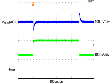
MAXM15065 LOAD TRANSIENT RESPONSE V_{IN} = 24V , FIXED V_{OUT} = 3.3V , PWM MODE (LOAD CURRENT STEPPED FROM 150mA TO 300mA)
