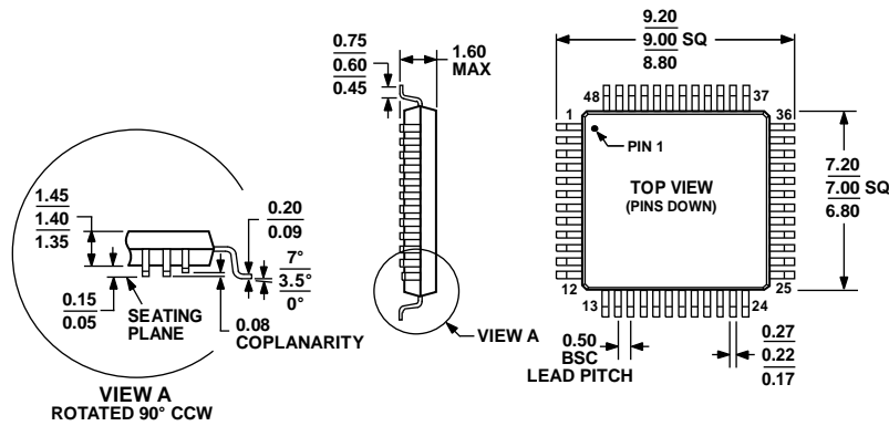
COMPLIANT TO JEDEC STANDARDS MS-026-BBC Figure 29. 48-Lead Low Profile Quad Flat Package [LQFP] (ST-48) Dimensions shown in millimeters
