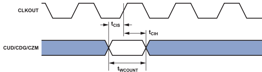
Figure 31. Up/Down Counter/Rotary Encoder Timing
