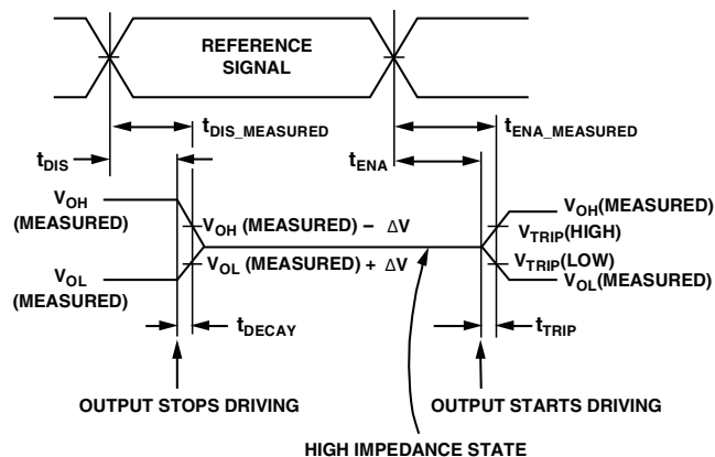
Figure 55. Output Enable/Disable
