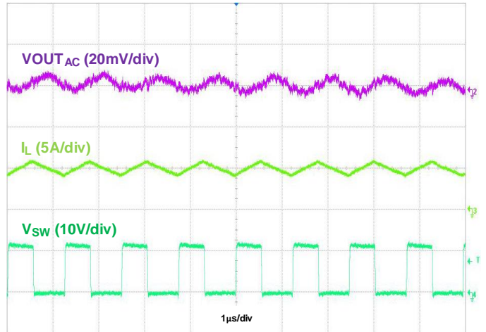
Figure 31. Output Voltage Ripple, VOUT = 5V, IOU = 5A
