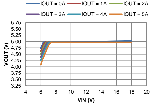
Figure 26. Line Regulation
