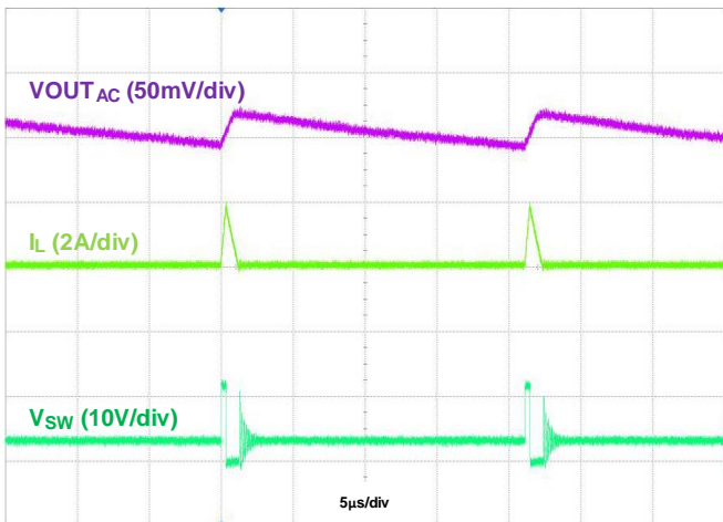
Figure 32. Output Voltage Ripple, VOUT = 3.3V, IOU = 50mA
