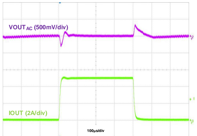
Figure 35. Load Transient, IOU = 50mA to 5A to 50mA
