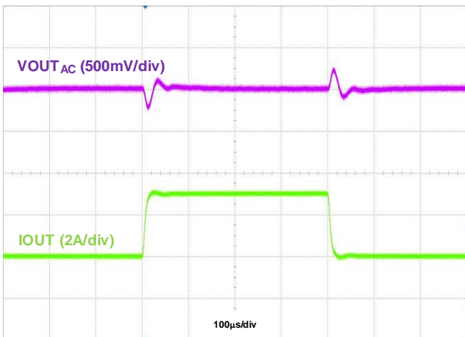
Figure 34. Load Transient, IOU = 2A to 5A to 4A
