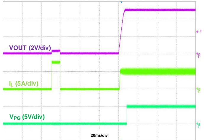
Figure 13. Output Short Recovery, I_{OUT} = 5\text{A}
