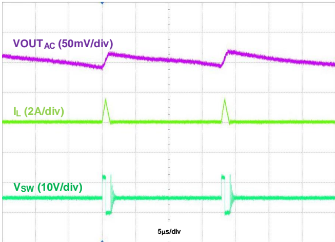
Figure 30. Output Voltage Ripple, VOUT = 5V, IOU = 50mA
