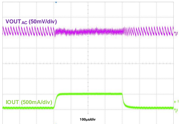
Figure 33. Load Transient, IOU = 50mA to 500mA to 50mA
