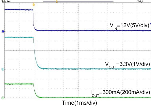
Power Off V_{OUT}=3.3V
