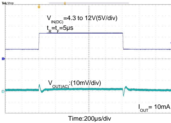
Line Transient Response V_{OUT}=3.3V
