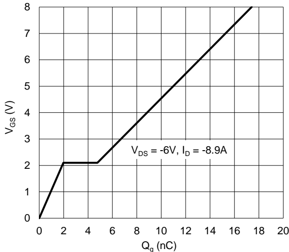
Figure 24. Gate Charge
