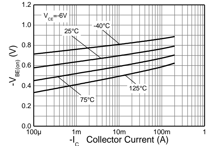
Figure 16. V_{BE(on)} v I_C
