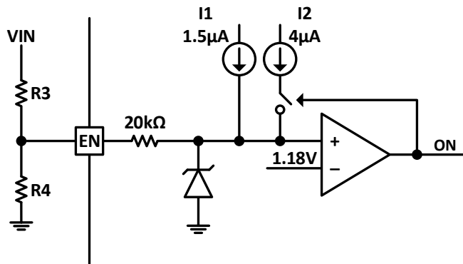
Figure 23. Programming UVLO
