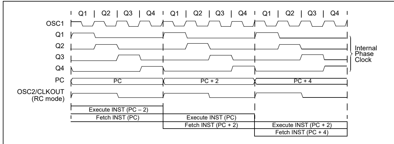
FIGURE 4-2: CLOCK/INSTRUCTION CYCLE
