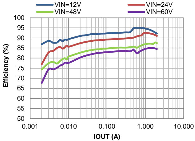
Figure 5. PFM Efficiency vs. Output Current, V_{OUT}=5\text{V} , L=10\mu\text{H}
