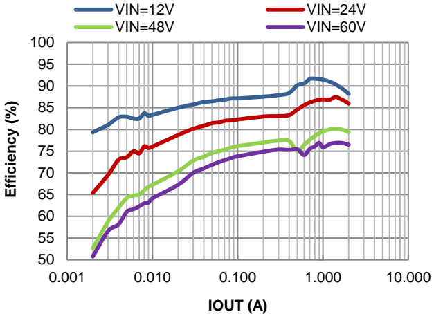
Figure 7. PFM Efficiency vs. Output Current, V_{OUT}=3.3\text{V} , L=8.2\mu\text{H}
