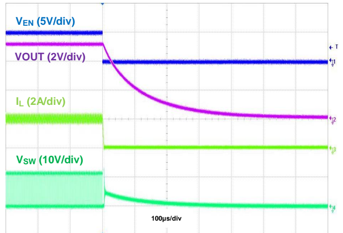
Figure 32. Shutdown using EN, IOUT = 2A
