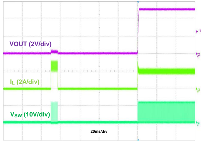
Figure 36. Output Short Recovery, I_{OUT} = 2\text{A}
