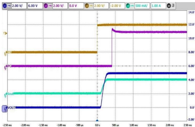
Turn On Response V_{IN} = 5V , V_{CC} = 5V , V_{EN} = 0V to 5V , R_L = 10\Omega
