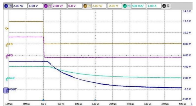
Turn Off Response V_{IN} = 5V , V_{CC} = 3.3V , V_{EN} = 0V to 3.3V , R_L = 10\Omega
