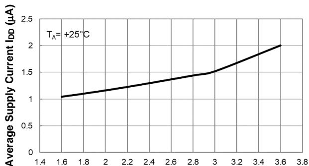
Supply voltage (V) Average Supply Current vs. Supply Voltage
