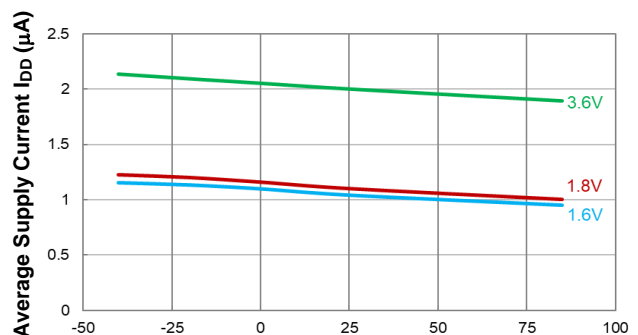
Temperature (°C) Average Supply Current vs. Temperature
