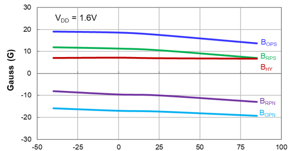
Temperature (°C) Switch Points B_{OPS} and B_{RPS} vs Temperature
