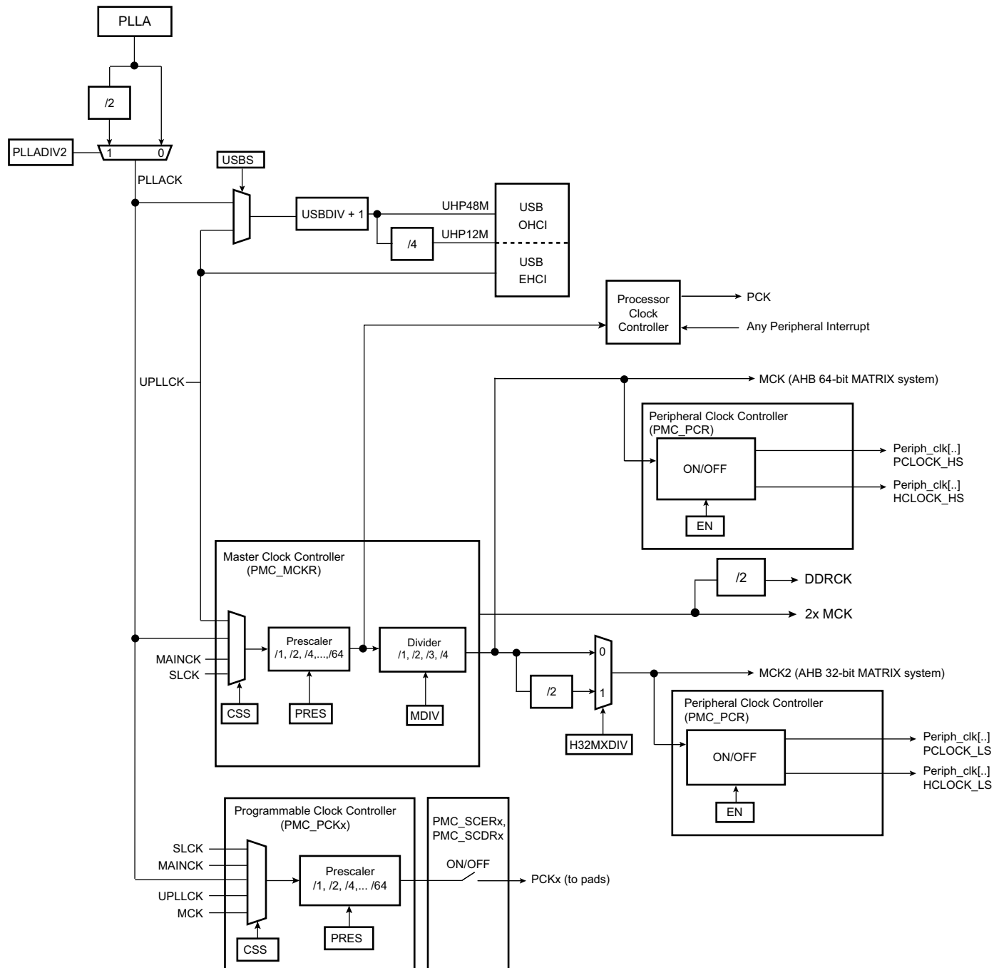
Figure 27-1: General Clock Block Diagram
