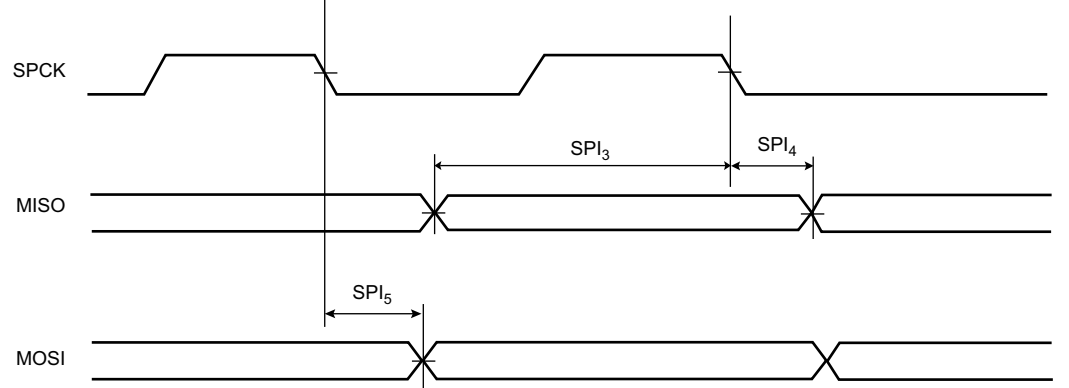
Figure 56-7: SPI Host Mode 0 and 3
