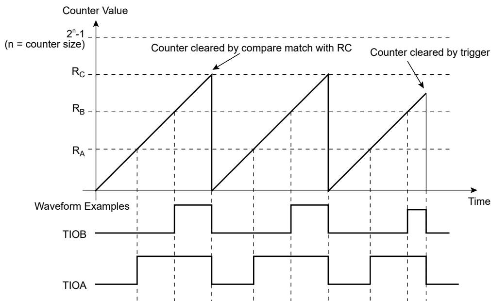
Figure 46-10: WAVSEL = 10 with Trigger
