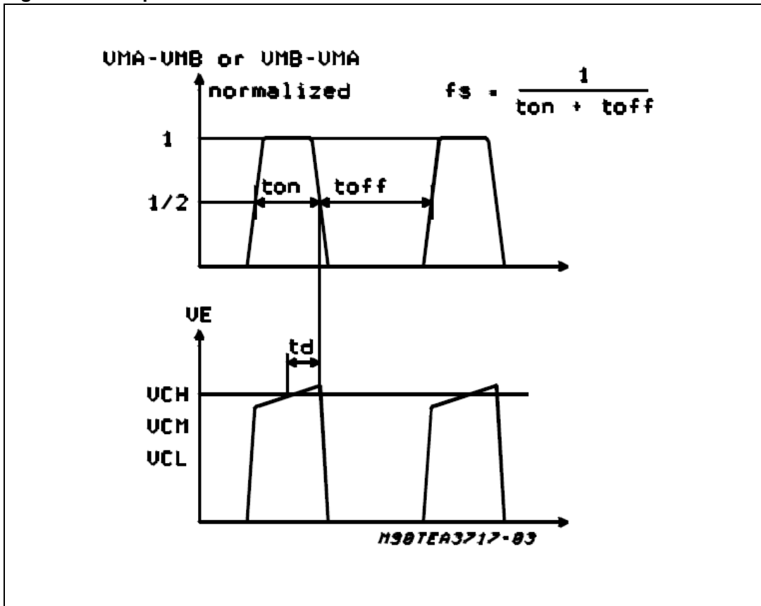
Figure 7. Output waveforms
