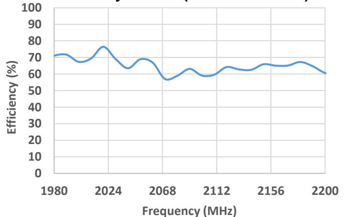
Efficiency S-Band (1980 – 2200 MHz)
