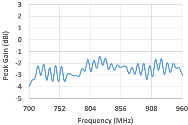
Peak Gain Low Band (700 – 960 MHz)
