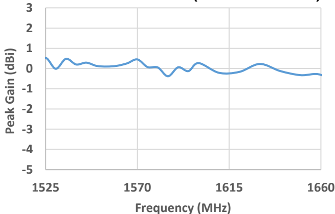
Peak Gain L-Band (1525 – 1660 MHz)
