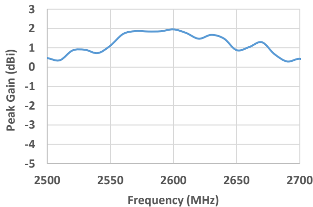
Peak Gain High Band (2500 – 2700 MHz)
