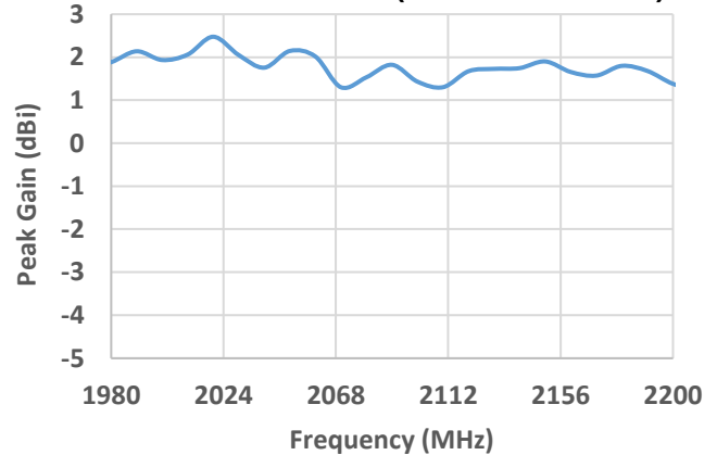
Peak Gain S-Band (1980 – 2200 MHz)
