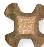
Indenter Crimp Cross-Section Across Axis
