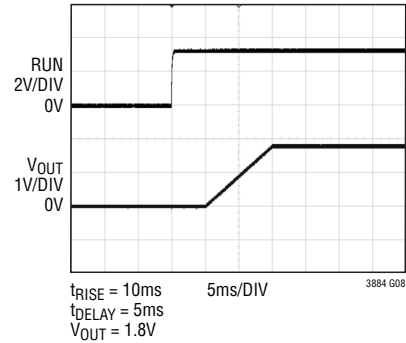
Soft-Start Ramp
