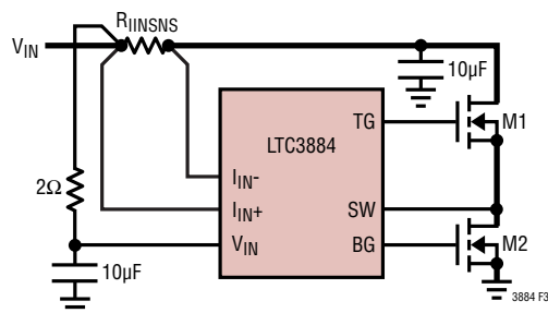
Figure 36. Low Noise Input Current Sense Circuit
