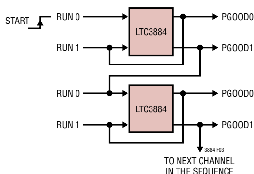
Voltage-Based Sequencing by Cascading PGs Into RUN Pins
