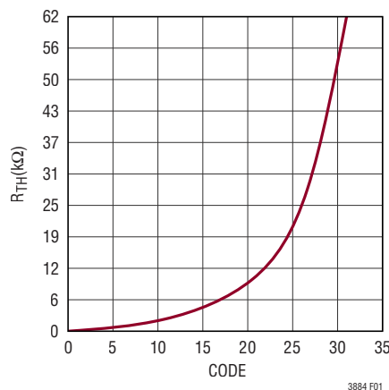
Figure 1. Programmable R_{TH}
