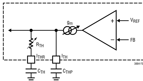
Figure 37. Programmable Loop Compensation
