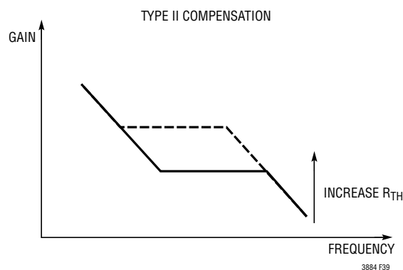
Figure 39. R_{TH} Adjust
