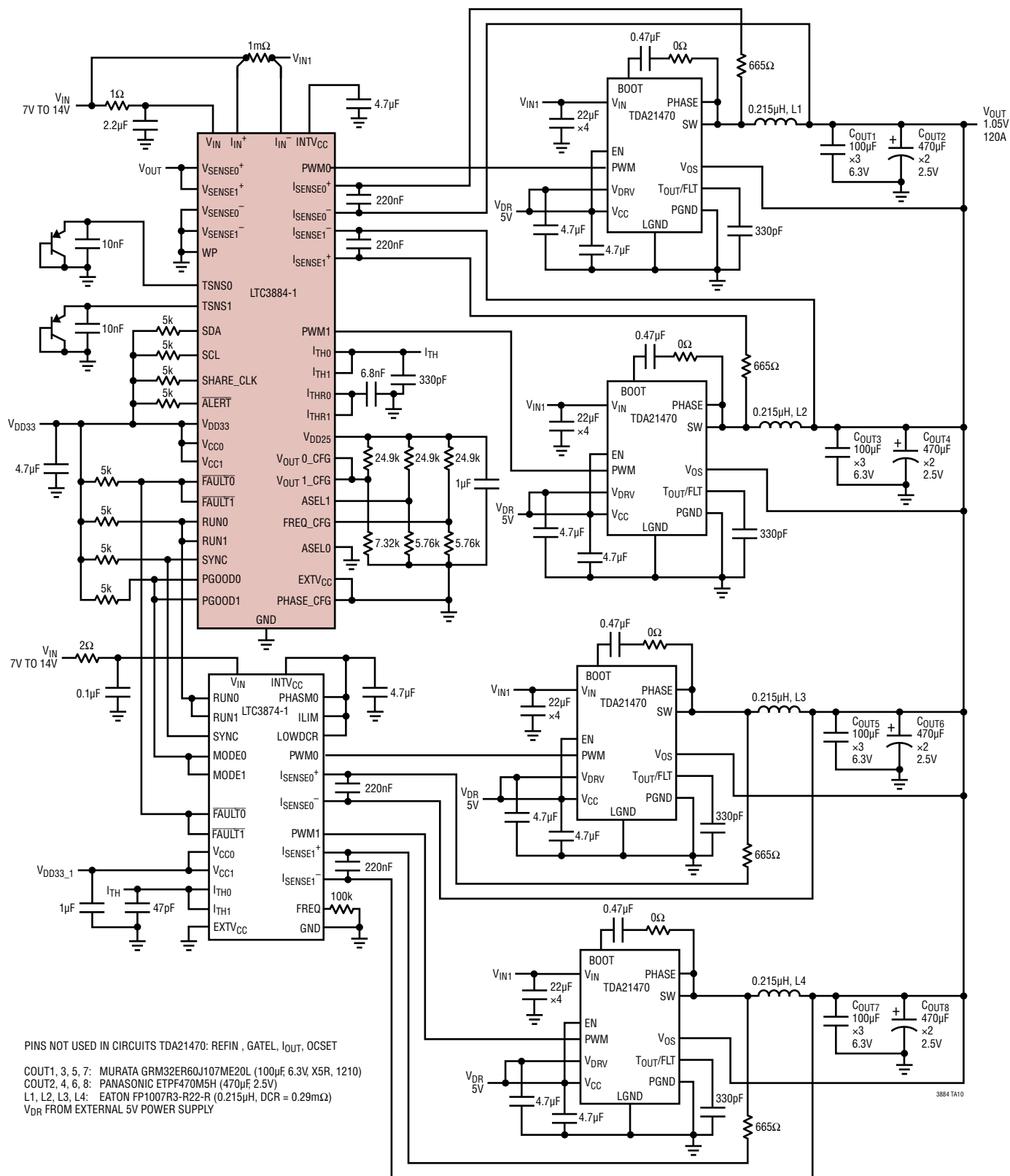
Low DCR Sensing, 500kHz 4-Phase 1.05 Step-Down Converter
