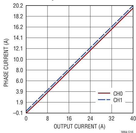
Phase Current Matching in Two Phase Systems
