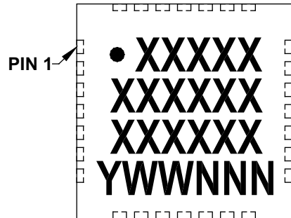
28-Lead VQFN
