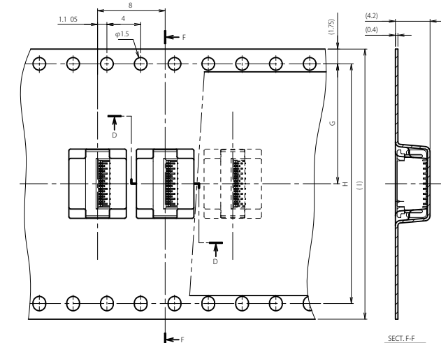
SECT. F-F
