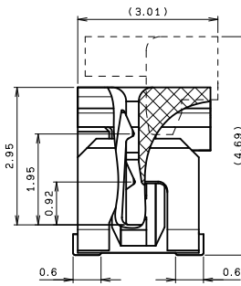
SECT. X-X
