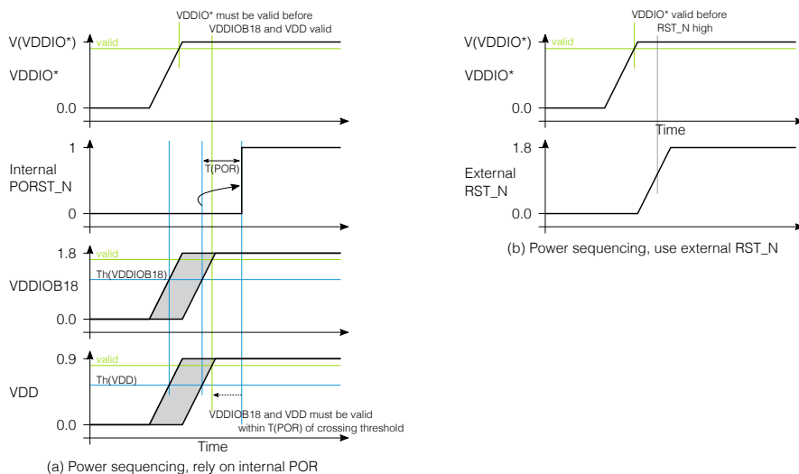
Figure 28: Sequencing of power supplies and RST_N (if used)
