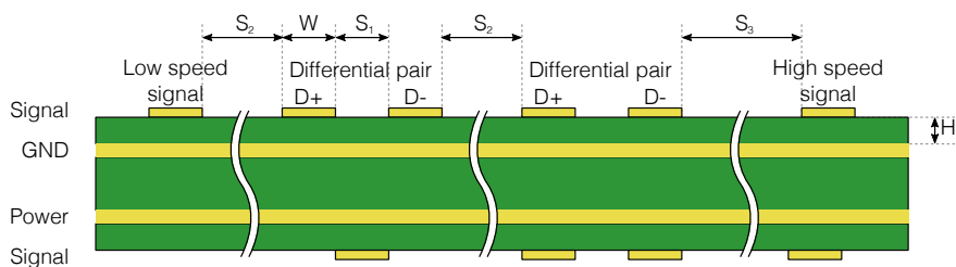
Figure 29: Spacings of a low speed signal, two differential pairs and a high speed signal
