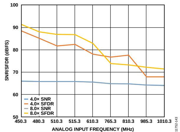
Figure 91. SNR/SFDR vs. f_{IN} ; 500 \text{ MHz} < f_{IN} < 1 \text{ GHz} ; Buffer Control 1 ( 0x018 ) = 4.0\times and 8.0\times
