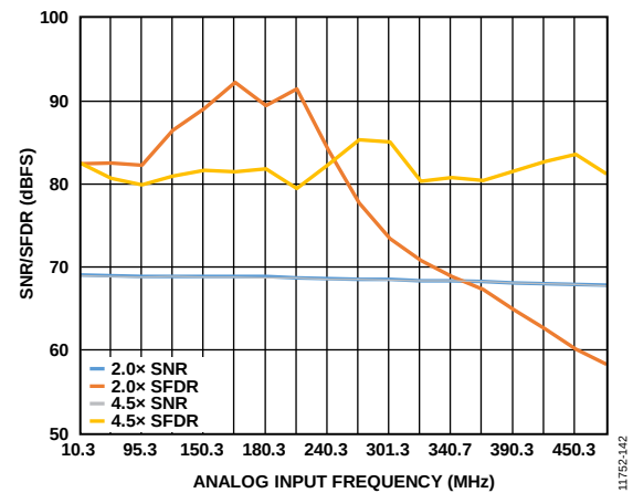
Figure 90. SNR/SFDR vs. f_{IN} ; f_{IN} < 500 MHz; Buffer Control 1 ( 0x018 ) = 2.0\times and 4.5\times
