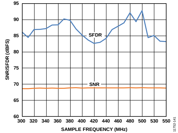
Figure 89. SNR/SFDR vs. f_s , f_{IN} = 170.3 MHz; Buffer Control 1 = 2.0\times
