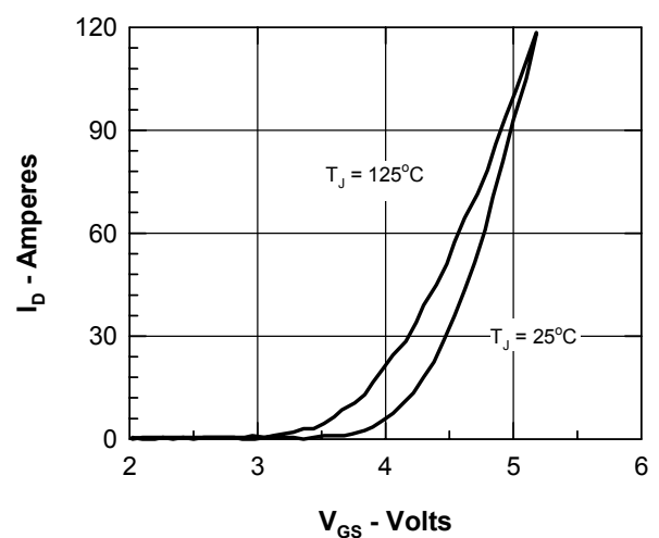
Figure 6. Admittance Curves
