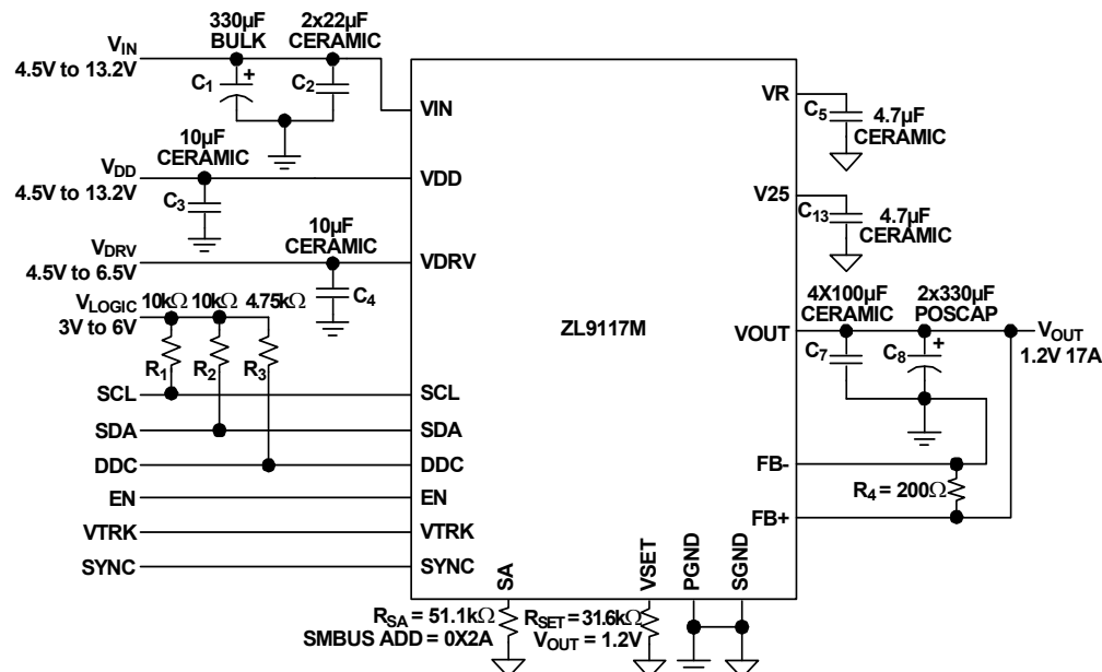
FIGURE 3. TYPICAL APPLICATION
