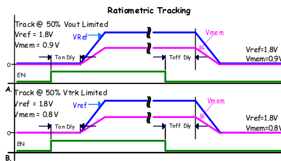
FIGURE 18. RATIOMETRIC TRACKING
