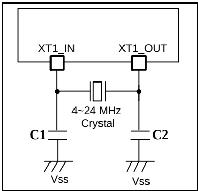
Figure 7.3-3 Typical HXT Crystal Application Circuit
