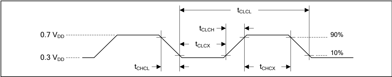
Figure 7.3-1 External 12 MHz High Speed Oscillator Timing Diagram
