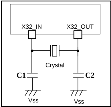
Figure 7.3-4 Typical LXT Crystal Application Circuit
