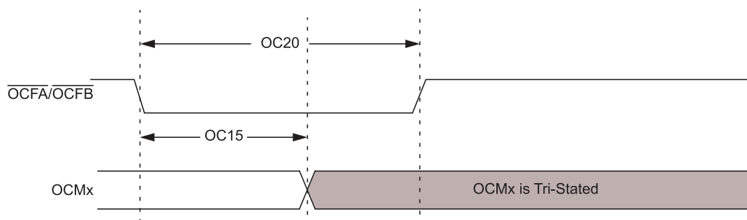
Figure 30-8. MCCP PWM Mode Timing Characteristics
