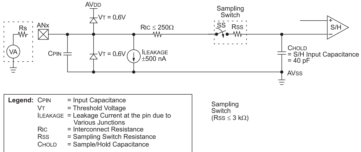
Figure 21-3. 12-Bit A/D Converter Analog Input Model
