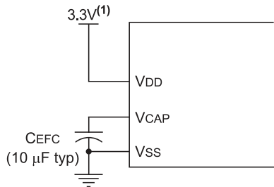
Figure 27-1. Connections for the On-Chip Regulator
