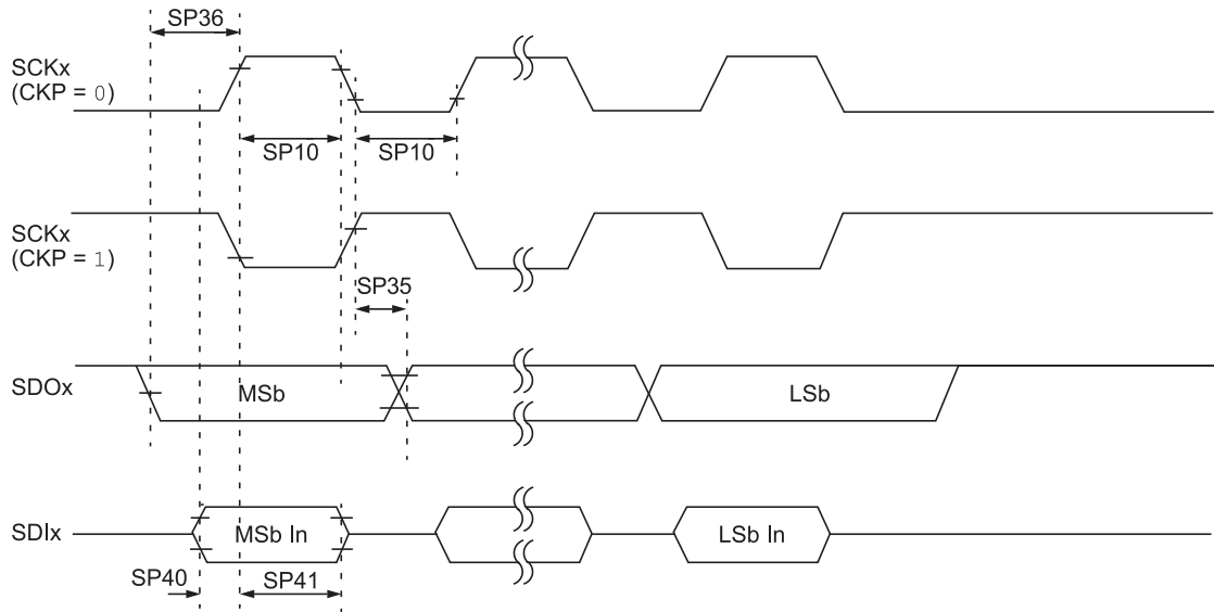
Figure 30-10. SPI Module Host Mode (CKE = 1) Timing Characteristics
