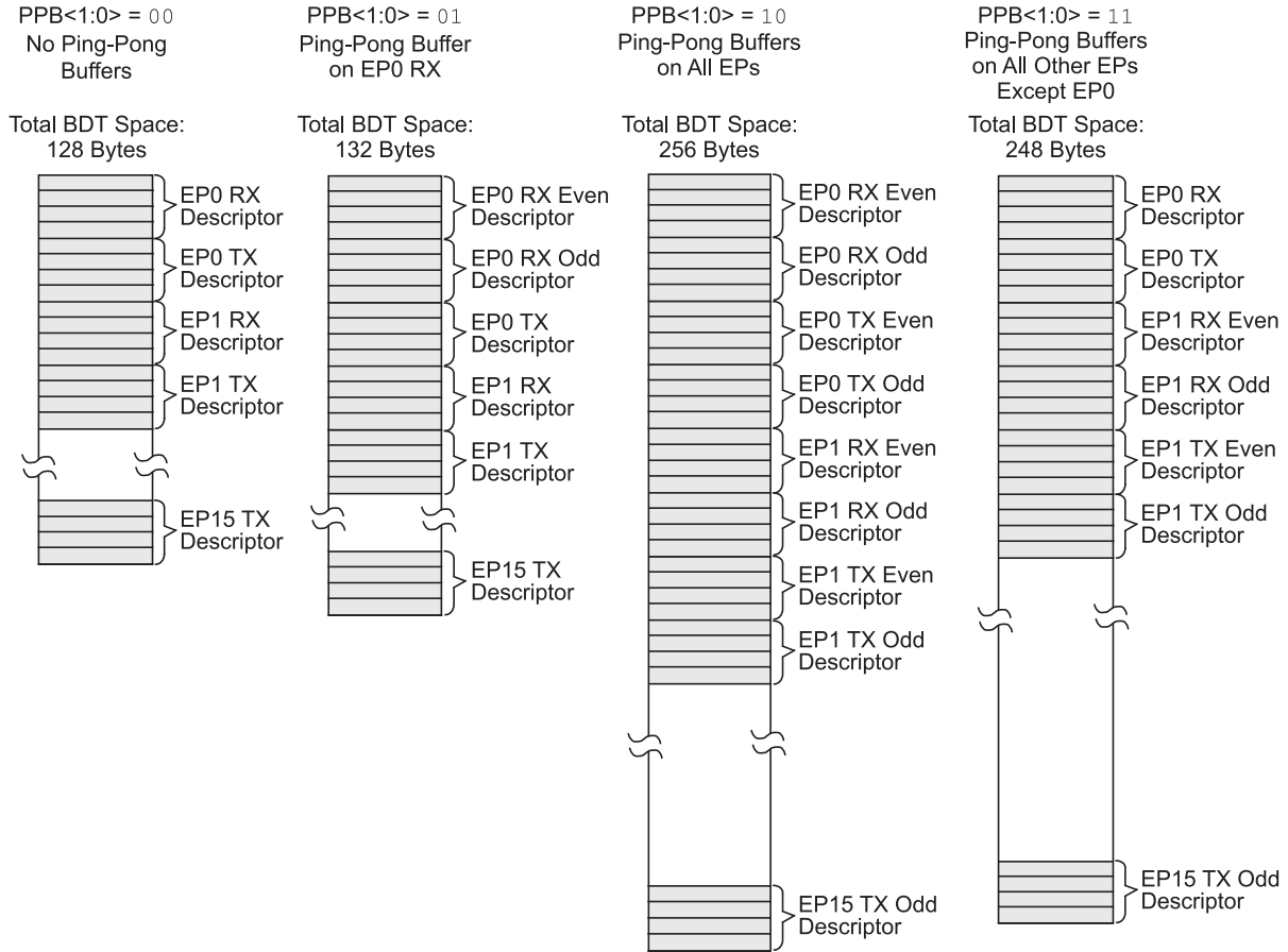
Figure 26-7. BDT Mapping for Endpoint Buffering Modes
