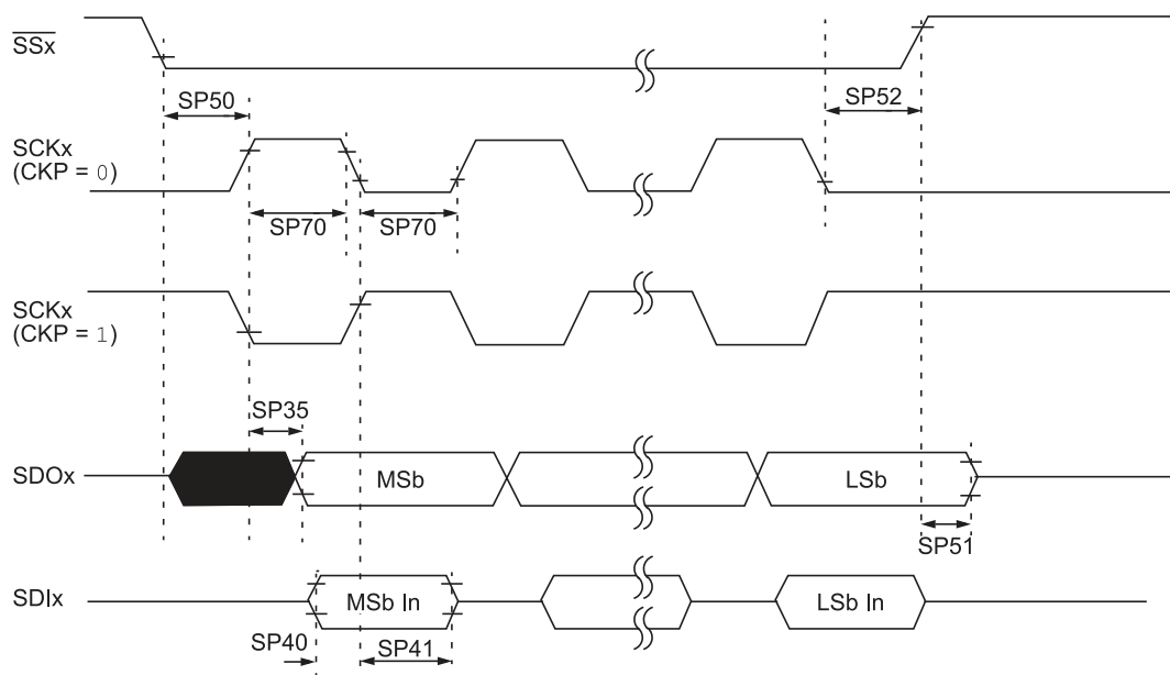
Figure 30-11. SPI Module Client Mode (CKE = 0) Timing Characteristics
